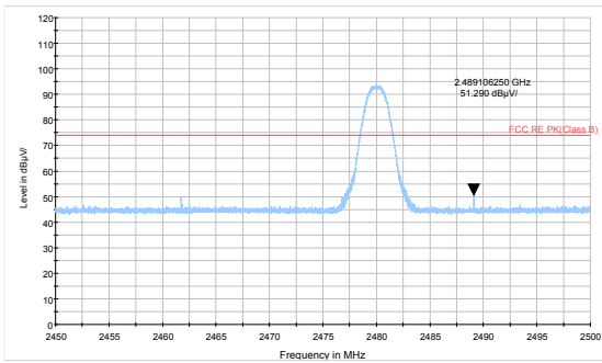
DH5-Channel 78: Peak
