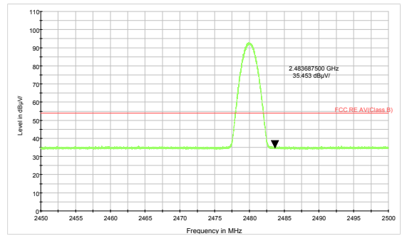
DH5-Channel 78: Average
