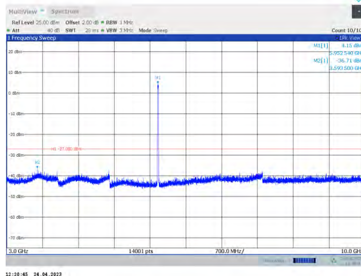
11a-CDD_Ant0_5955_3000~10000
