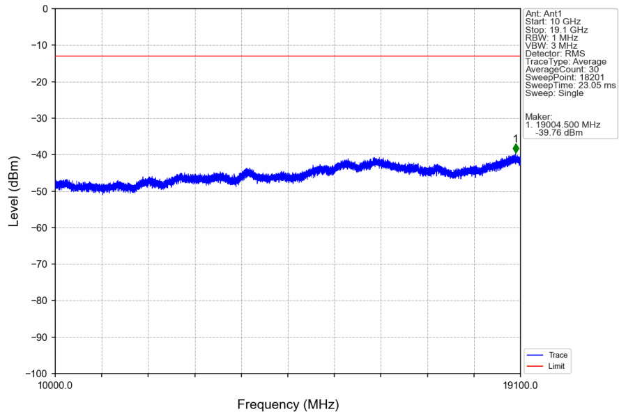
Band2_HSDPA_HCH_1907.6MHz_Subtest 1_NTNV
