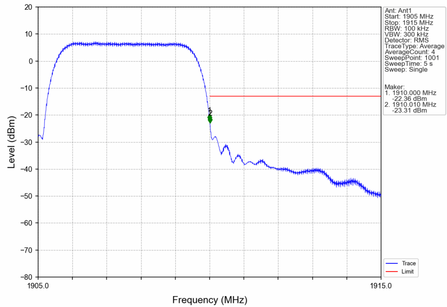
Band2_HSDPA_HCH_1907.6MHz_Subtest 1_NTNV
