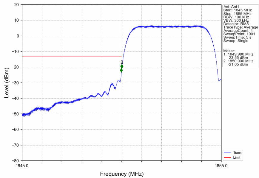
Band2_HSDPA_LCH_1852.4MHz_Subtest 1_NTNV
