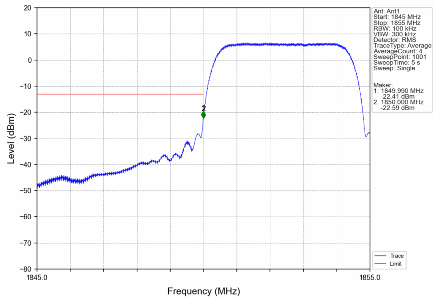
Band2_HSUPA_LCH_1852.4MHz_Subtest 1_NTNV
