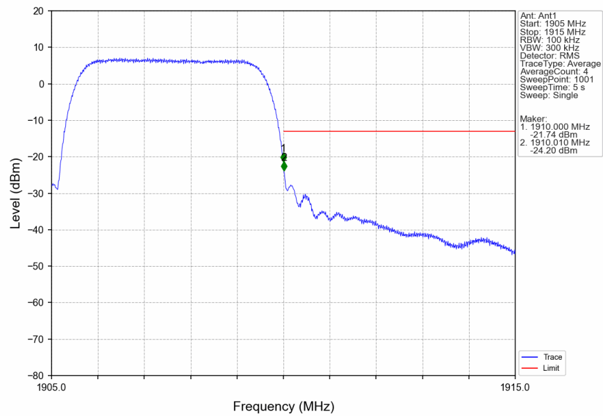
Band2_HSUPA_HCH_1907.6MHz_Subtest 1_NTNV
