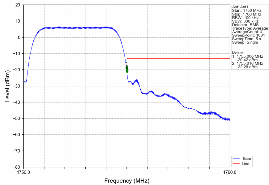
Band4_HSDPA_HCH_1752.6MHz_Subtest 1_NTNV
