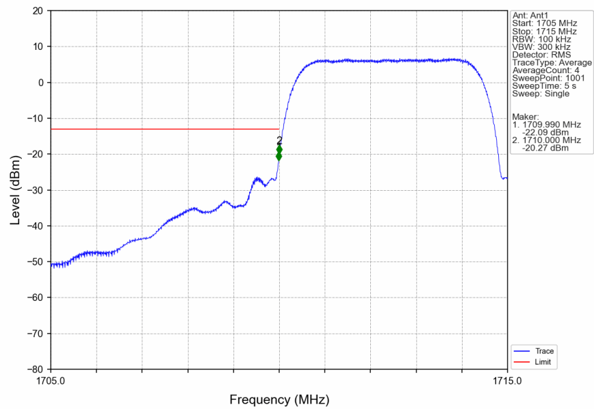
Band4_HSDPA_LCH_1712.4MHz_Subtest 1_NTNV
