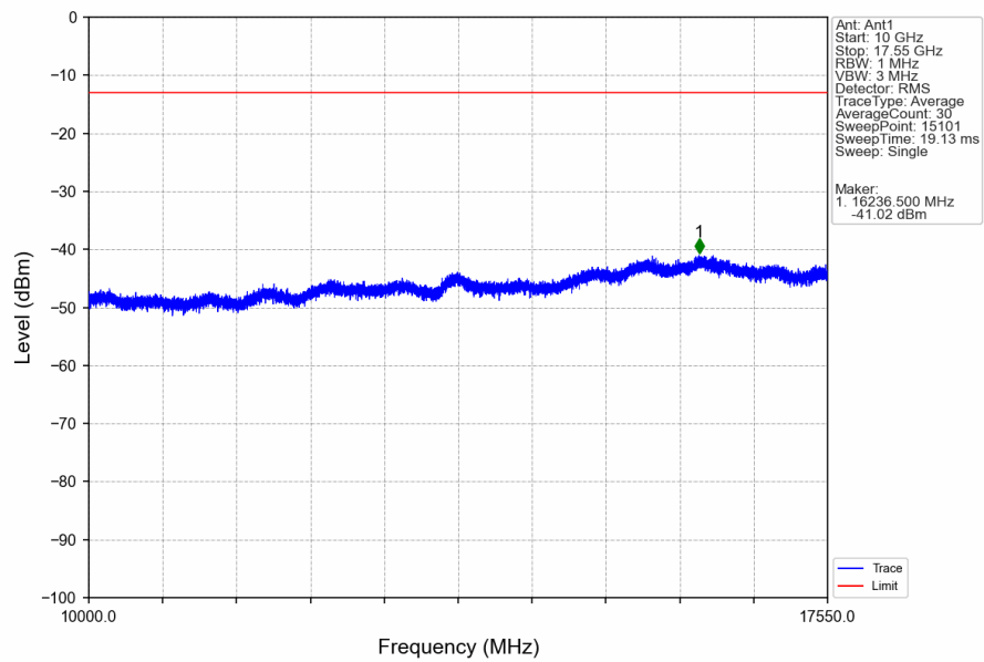
Band4_HSDPA_MCH_1732.6MHz_Subtest 1_NTNV
