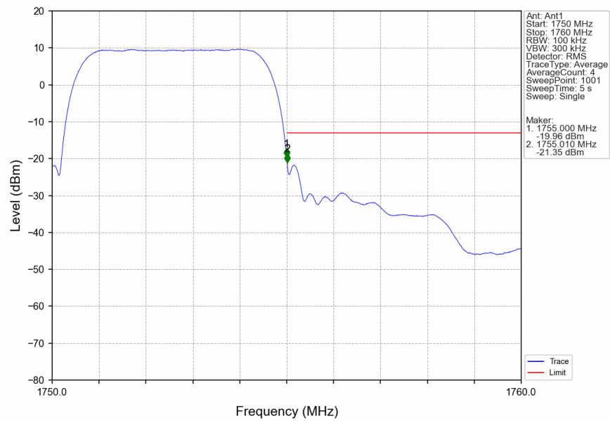
Band4_RMC_HCH_1752.6MHz_12.2kbps RMC_NTNV
