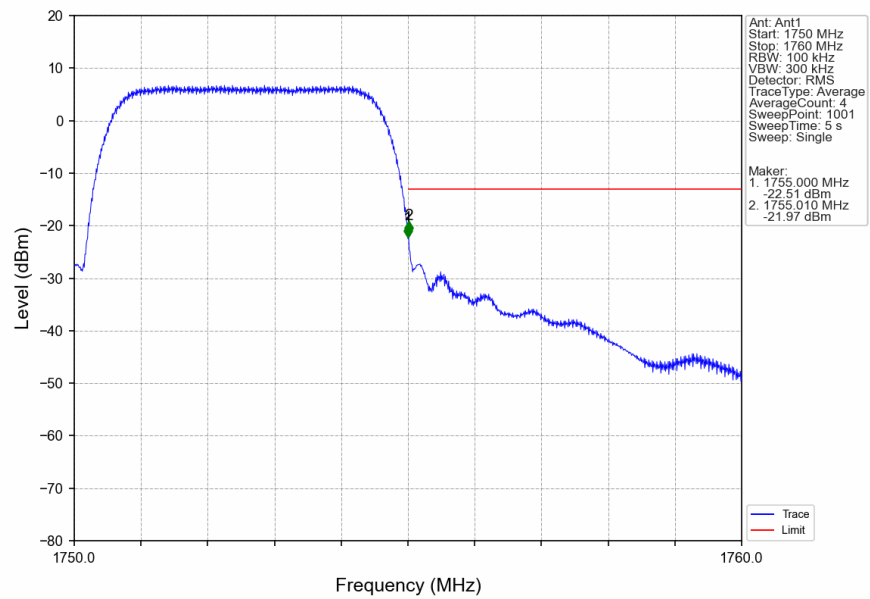
Band4_HSUPA_HCH_1752.6MHz_Subtest 1_NTNV
