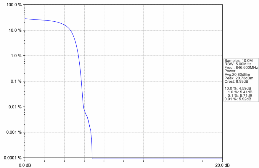
Band5_HSDPA_HCH_846.6MHz_Subtest 1_NTNV
