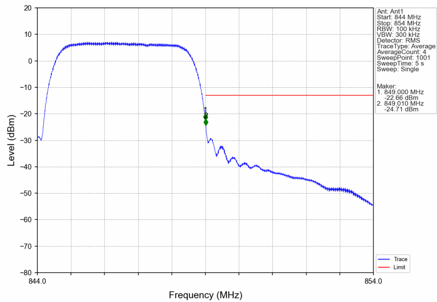
Band5_HSUPA_HCH_846.6MHz_Subtest 1_NTNV
