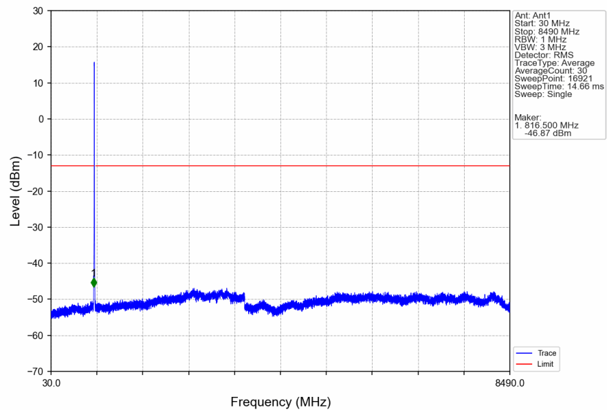
Band5_HSDPA_MCH_836.6MHz_Subtest 1_NTNV
