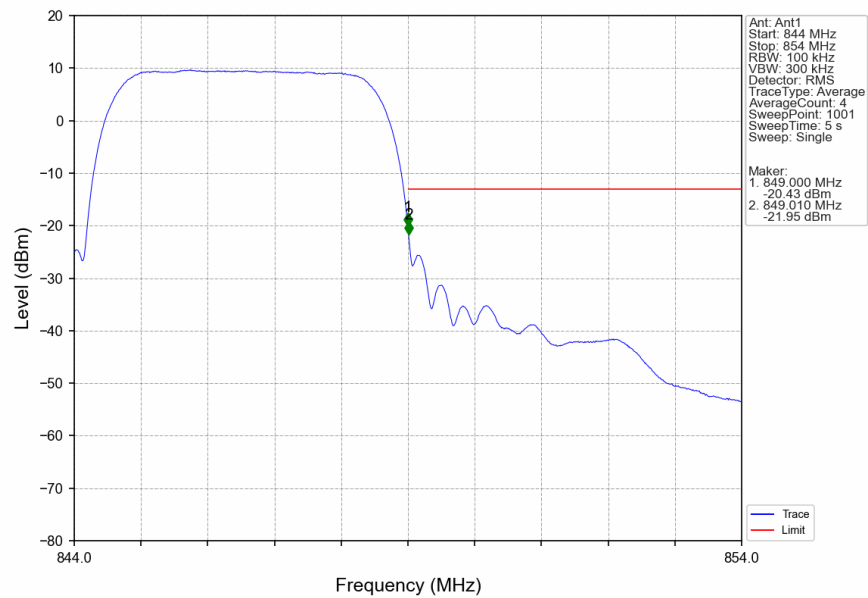
Band5_RMC_HCH_846.6MHz_12.2kbps RMC_NTNV
