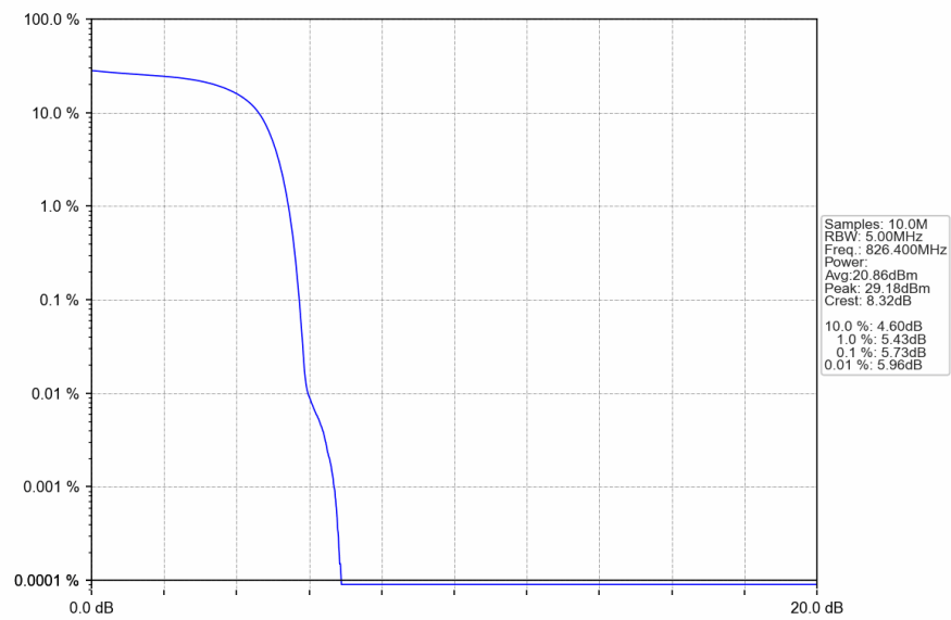
Band5_HSDPA_LCH_826.4MHz_Subtest 1_NTNV
