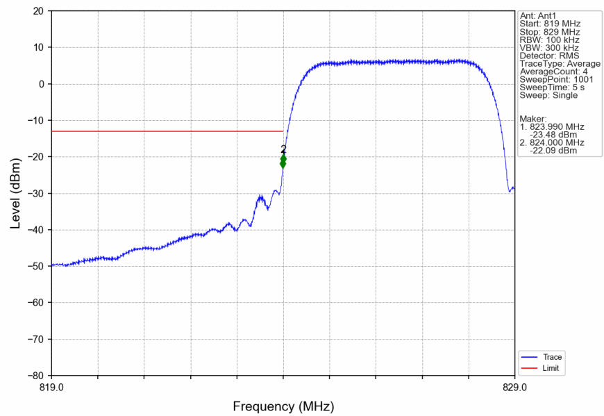
Band5_HSDPA_LCH_826.4MHz_Subtest 1_NTNV
