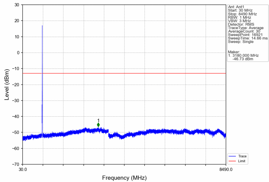
Band5_HSUPA_LCH_826.4MHz_Subtest 1_NTNV
