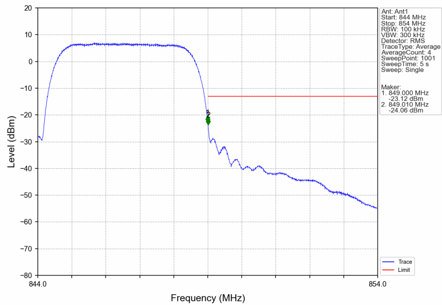
Band5_HSDPA_HCH_846.6MHz_Subtest 1_NTNV
