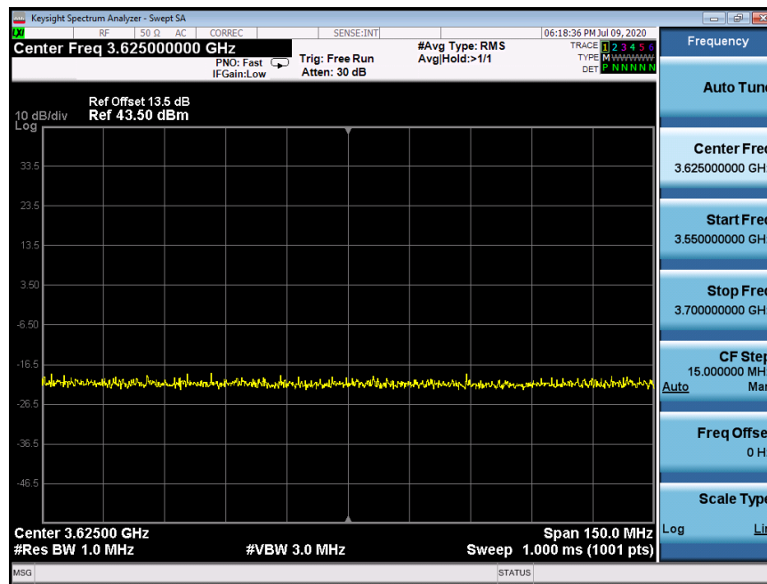
Plot 23. Conducted Measurement – No RF transmission in entire band at anytime (WINNF.FT.C.SCS.2)
