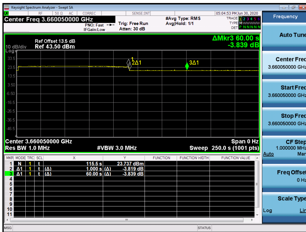
Plot 15. Conducted Measurement - RF transmission stops within 60s of SAS message. The SAS message is indicated by Marker 1 (WINNF.FT.D.HBT.8)
