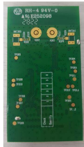
Fig 5.2 5G_MODULE_FPC Module TX Button ViewTop View
