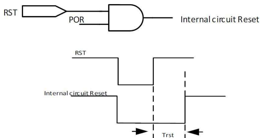
Fig 4.1 Power On Reset Timing Chart
