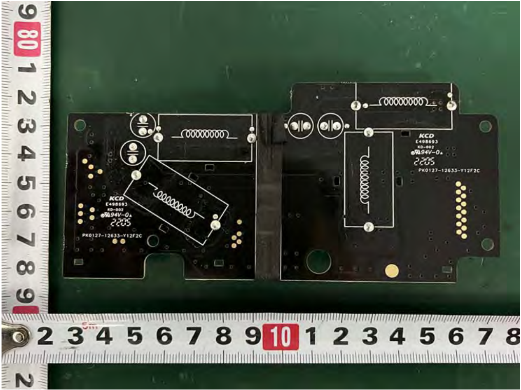
Internal Photos M/N: M512E-K6
