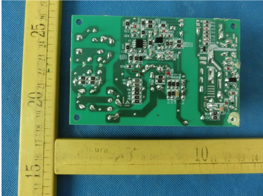
Photo 9 (Power Panel2)
