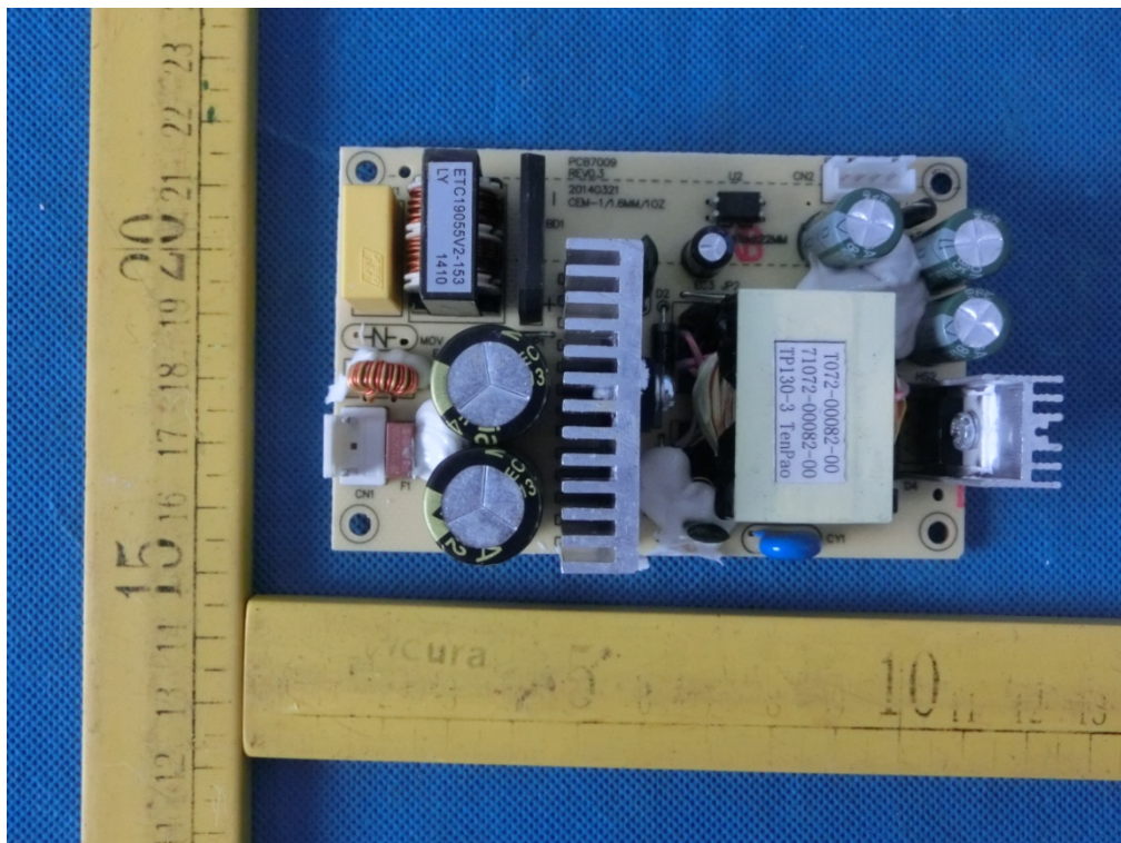
Photo 6 (Power Panel1)
