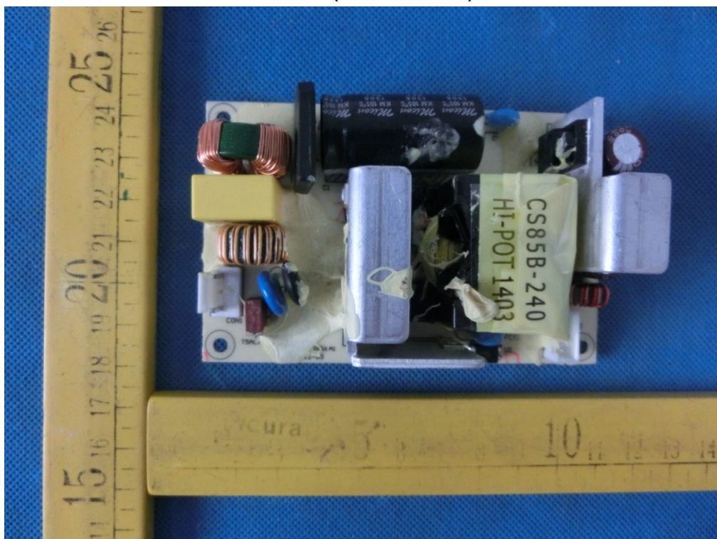
Photo 8 (Power Panel2)
