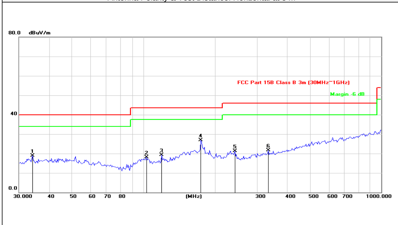
Antenna Polarity & Test Distance: Horizontal at 3 m
