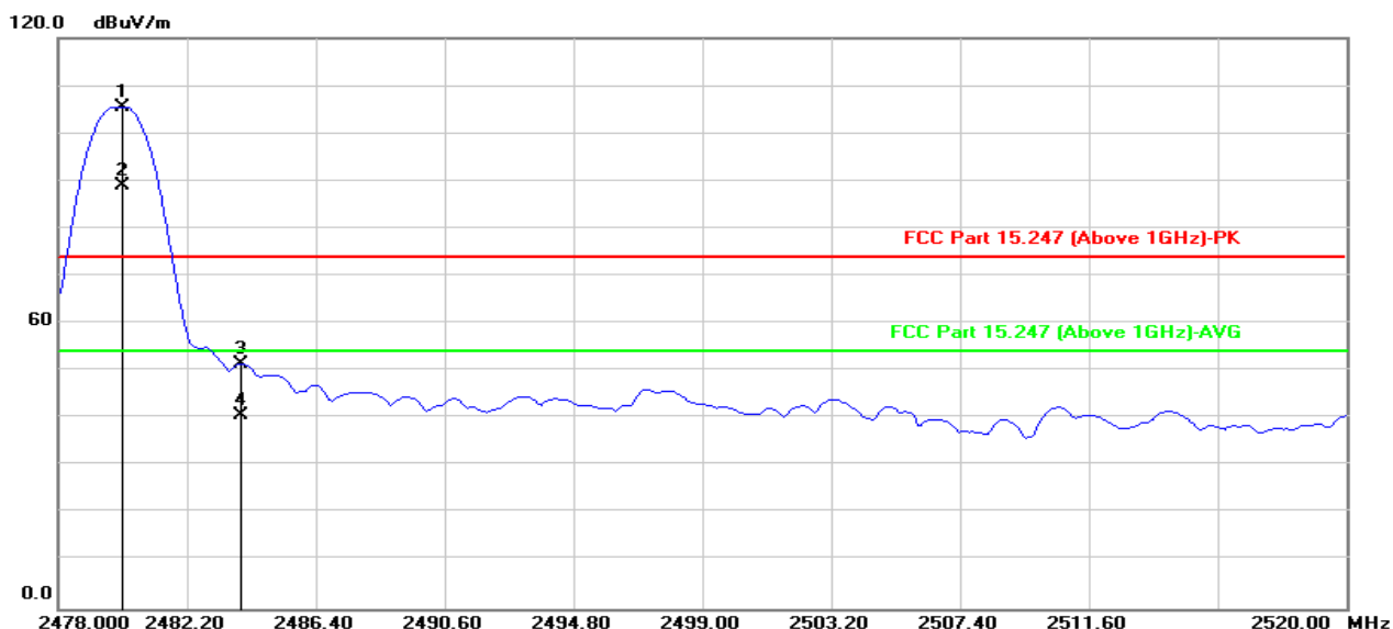
Antenna Polarity &amp; Test Distance: Horizontal at 3 m
