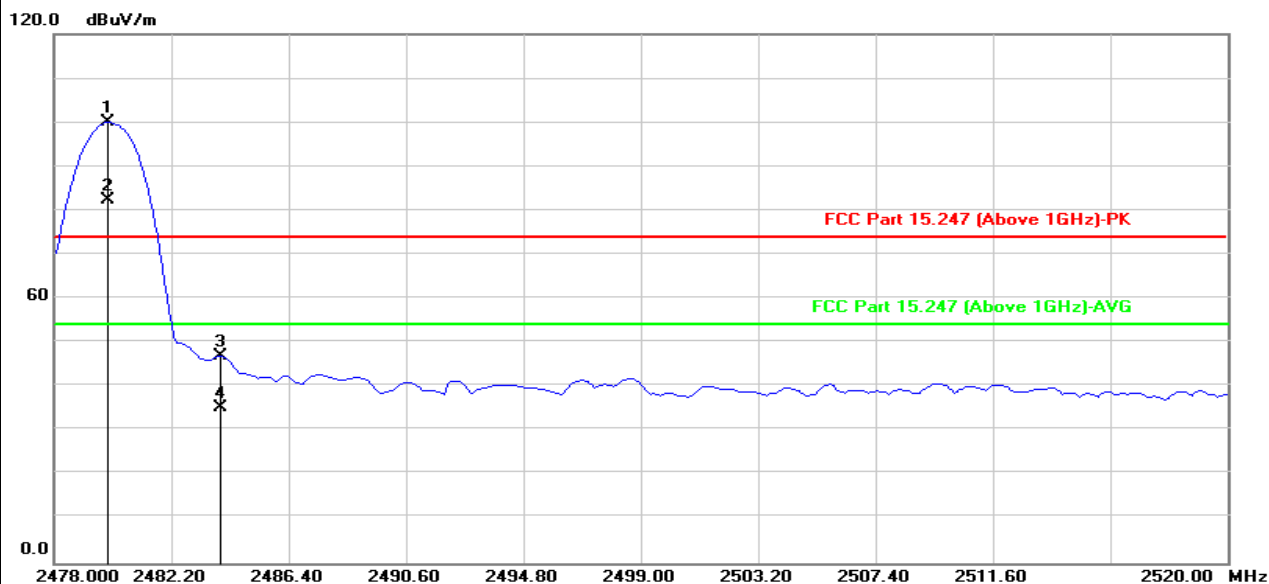
Antenna Polarity &amp; Test Distance: Vertical at 3 m
