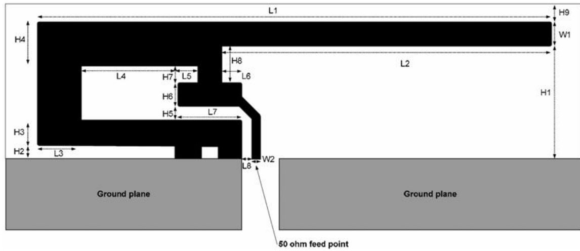
Figure 1-1. IFA Dimensions
