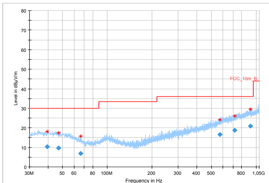
Plot 1: 30 MHz to 1 GHz, RX / idle – mode, vertical & horizontal polarization
