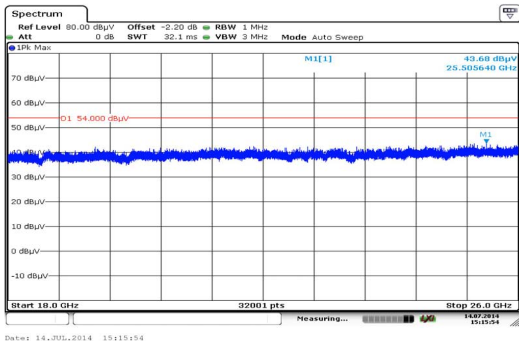
Plot 8: 18 GHz to 26 GHz, mid channel, vertical & horizontal polarization
