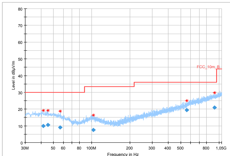
Plot 9: 30 MHz to 1 GHz, highest channel, vertical & horizontal polarization
