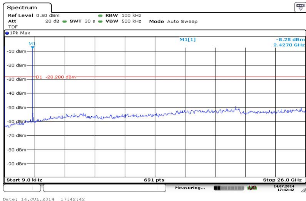
Plot 2: mid channel
