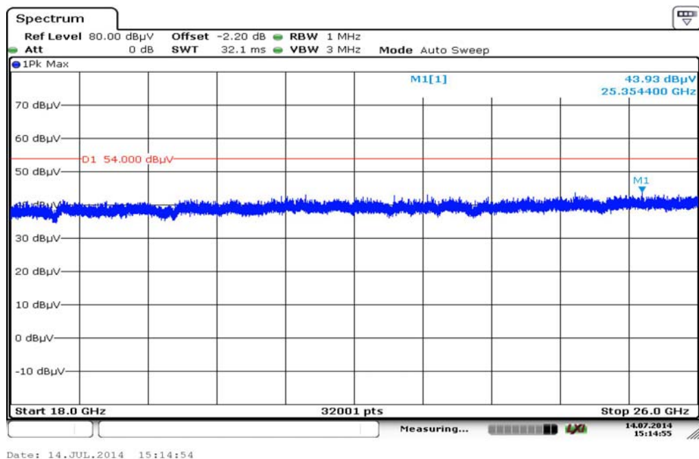
Plot 4: 18 GHz to 26 GHz, lowest channel, vertical & horizontal polarization
