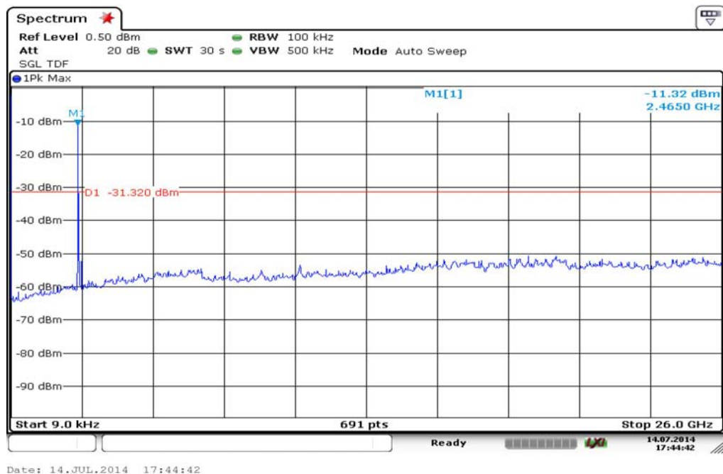
Plot 3: highest channel
