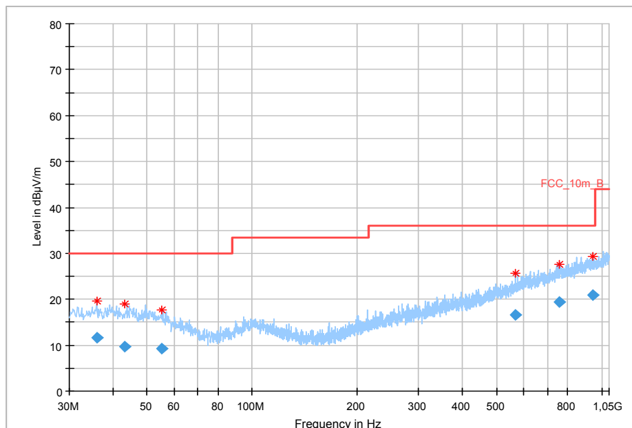
Plot 5: 30 MHz to 1 GHz, mid channel, vertical & horizontal polarization
