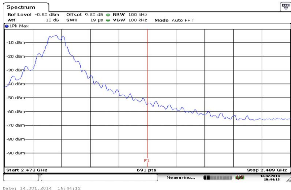
Plot 2: Upper band edge – hopping off
