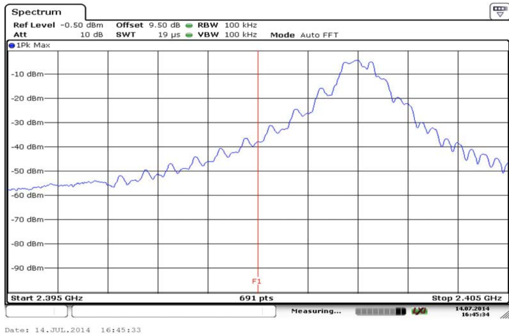
Plot 1: Lower band edge – hopping off
