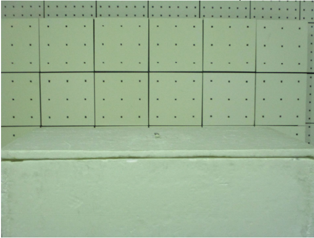
FCC_15_247_WLAN_Radiated_Setup
