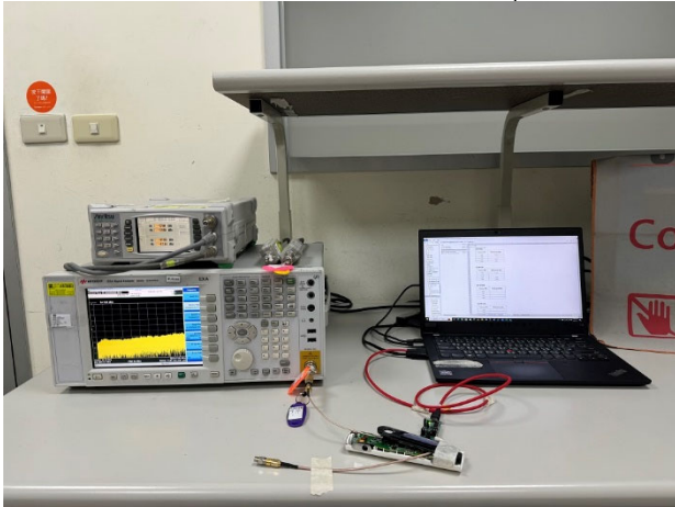
FCC_15_247_WLAN_Conducted_Setup
