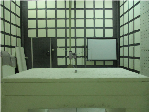
FCC_15_247_WLAN_Radiated_Setup
