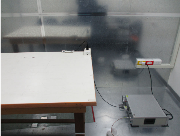
FCC_15_247_WLAN_Conduction_Setup
