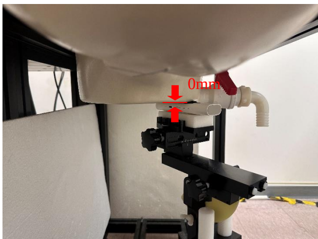
Photograph 1. Body, Front Surface, 0mm
