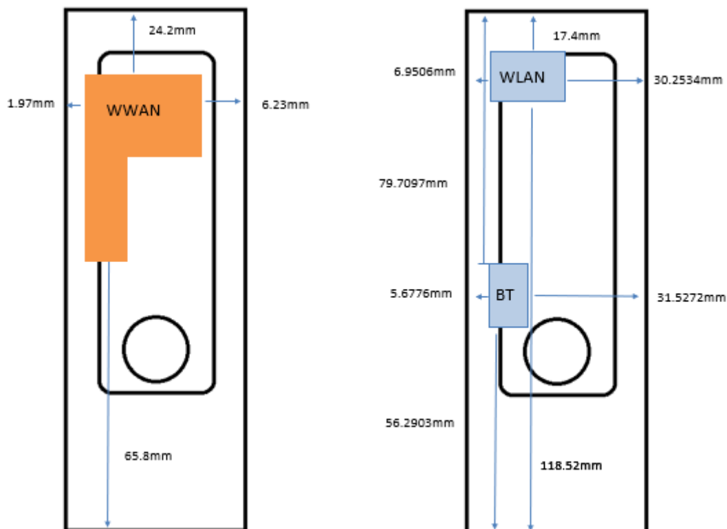
Photograph 15. Antenna position of EUT
