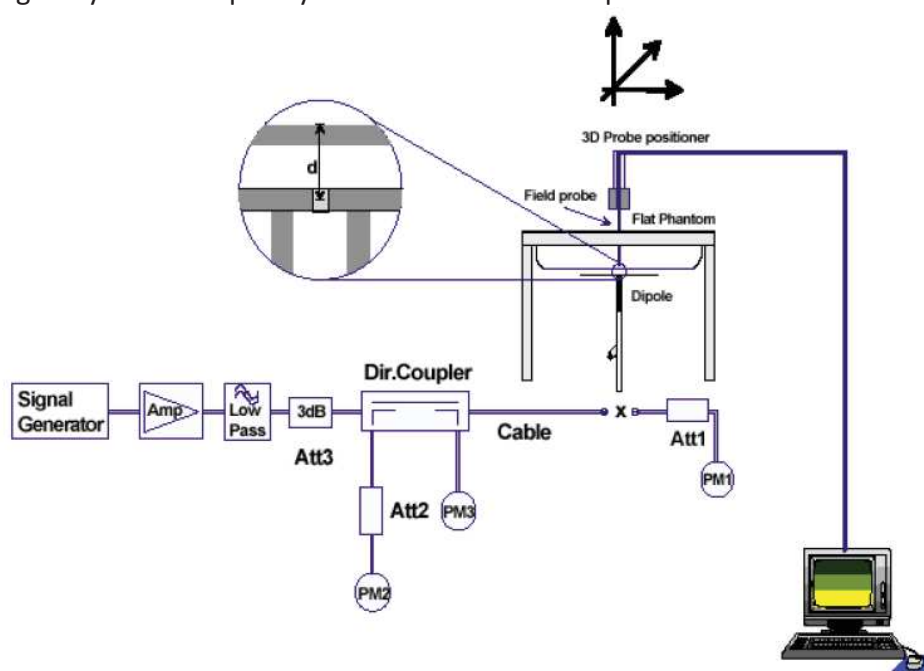
Picture 8: system Check Set-up
