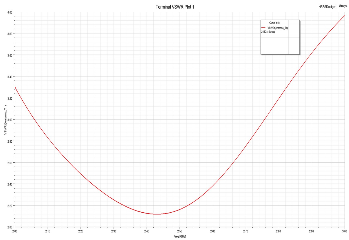
Figure 2: VSWR
