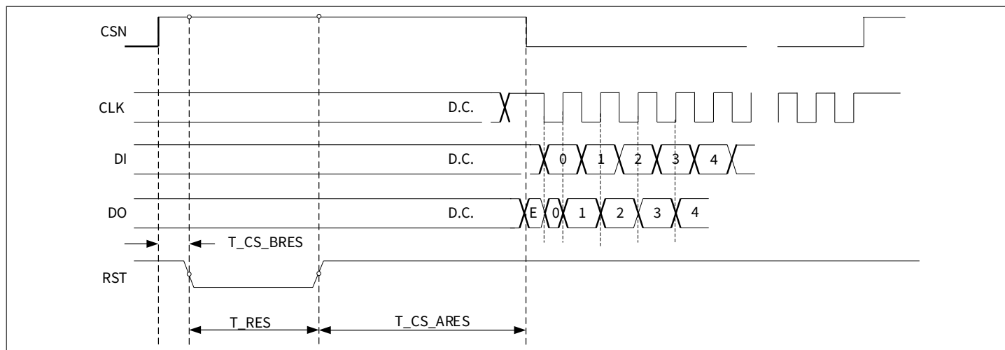
Figure 36 Hardware reset sequence
