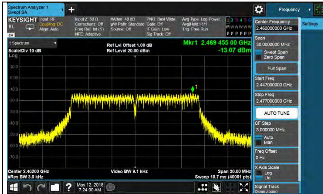
802.11g-2462MHz Chain 0
