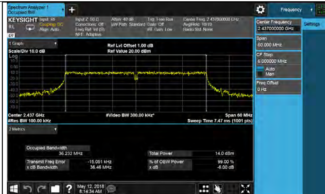
802.11n-HT40-2437MHz
