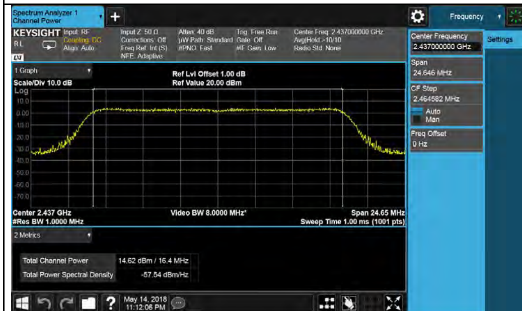
802.11g-2437MHz Chain 1
