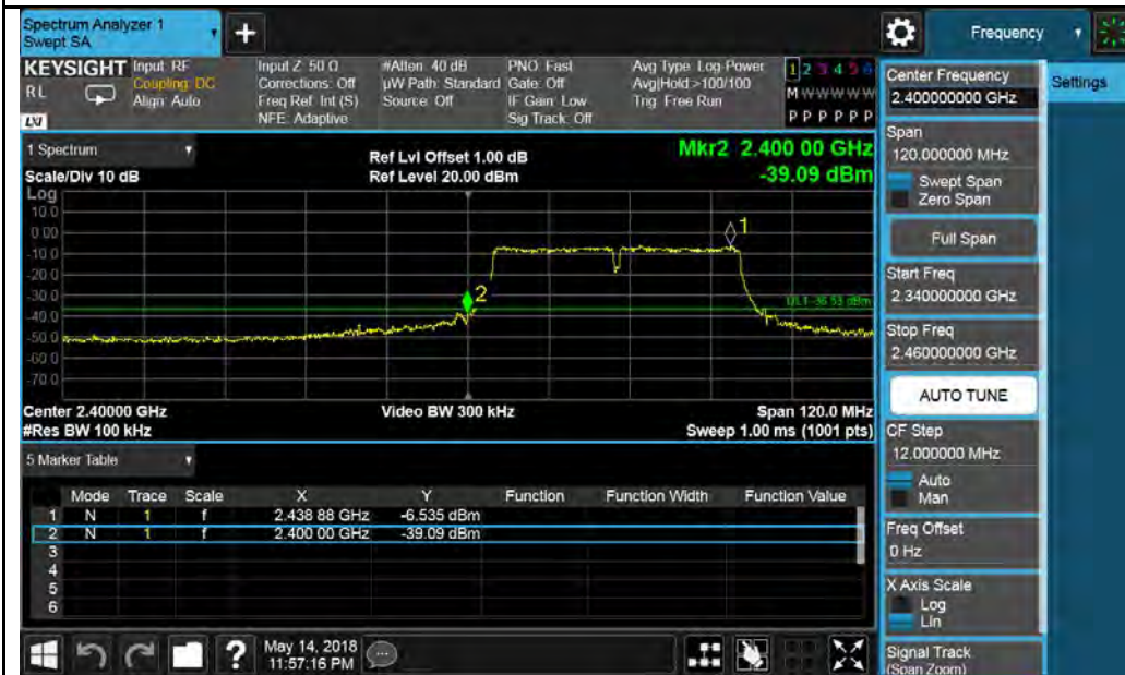
802.11n-HT40-2422MHz Chain 1
