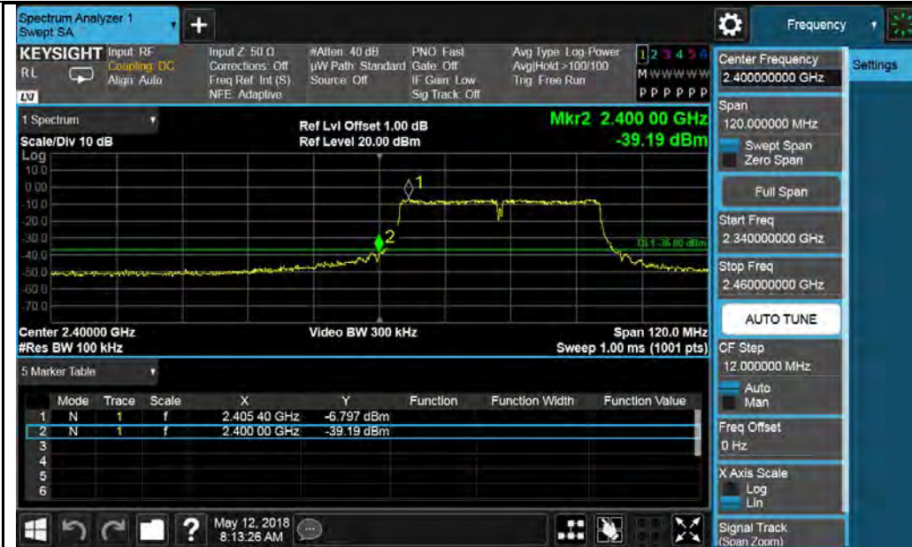
802.11n-HT40-2422MHz Chain 0
