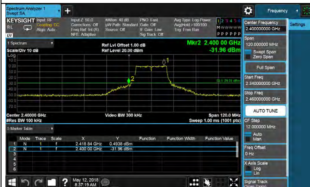
802.11g-2412MHz Chain 1
