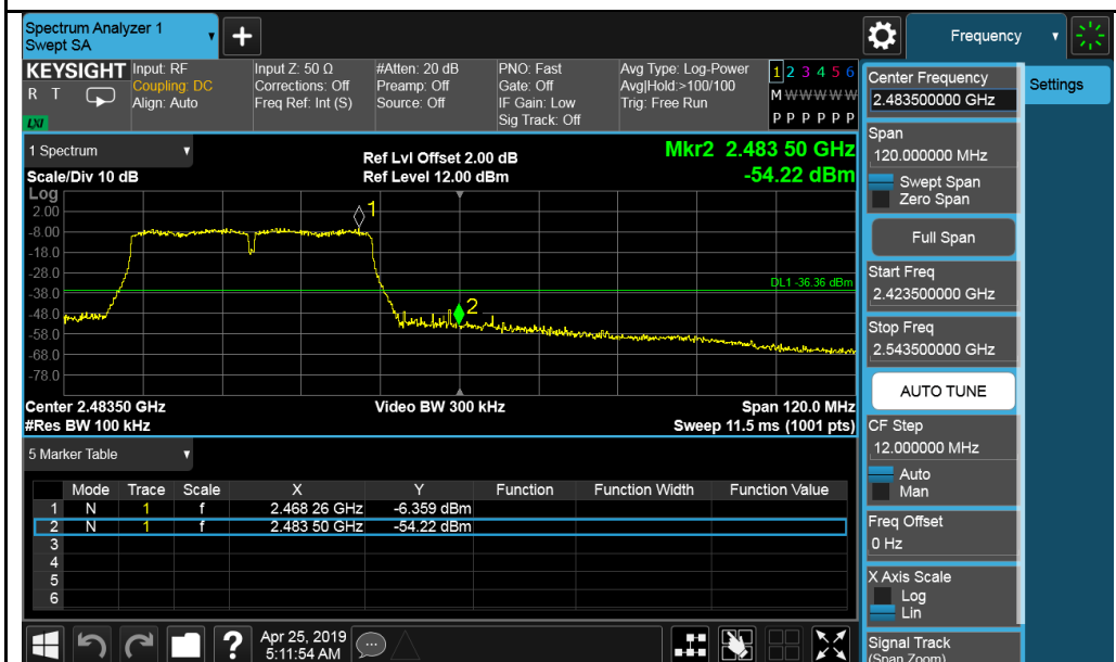
802.11n-HT40-2452MHz TX1
