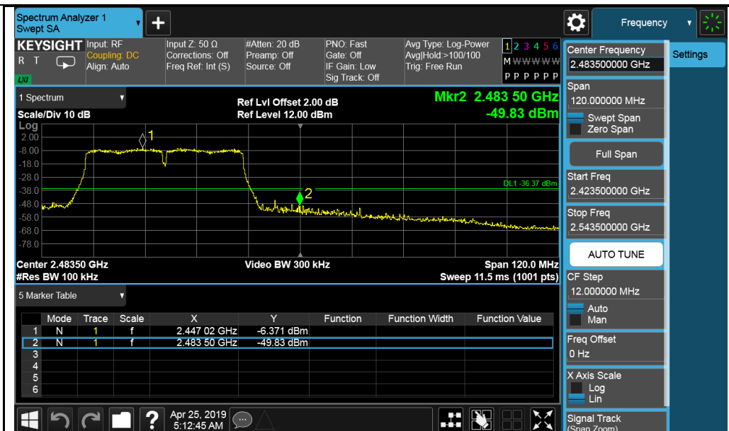
802.11n-HT40-2452MHz TX0
