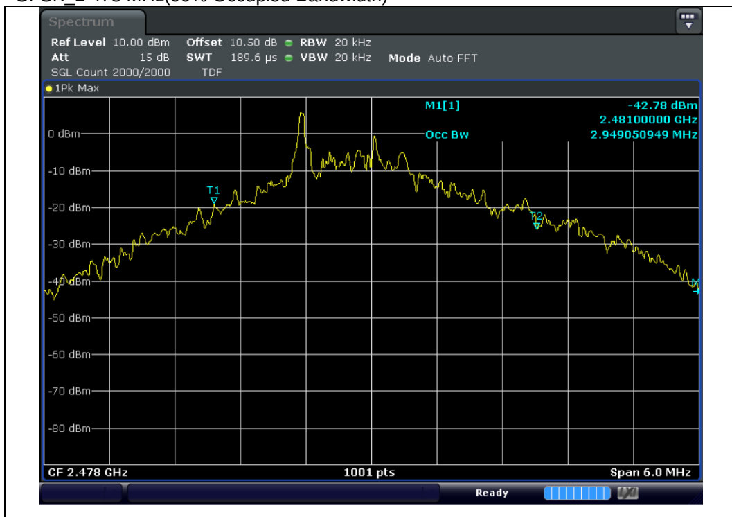
GFSK_2 478 MHz(99% Occupied Bandwidth)
