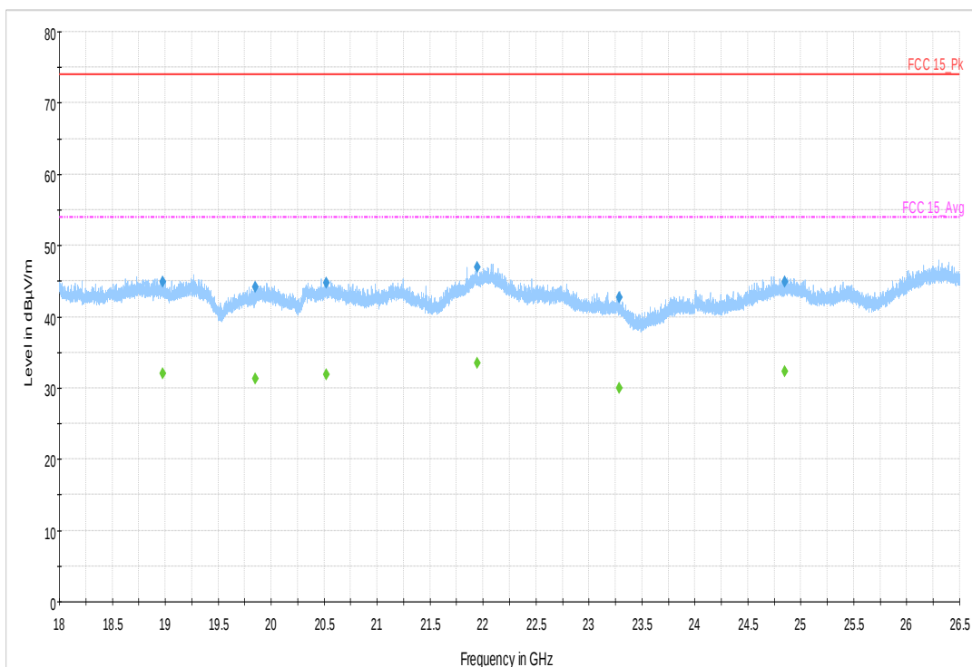
Plot 30. 18-26.5GHz, BLE-2440MHz
