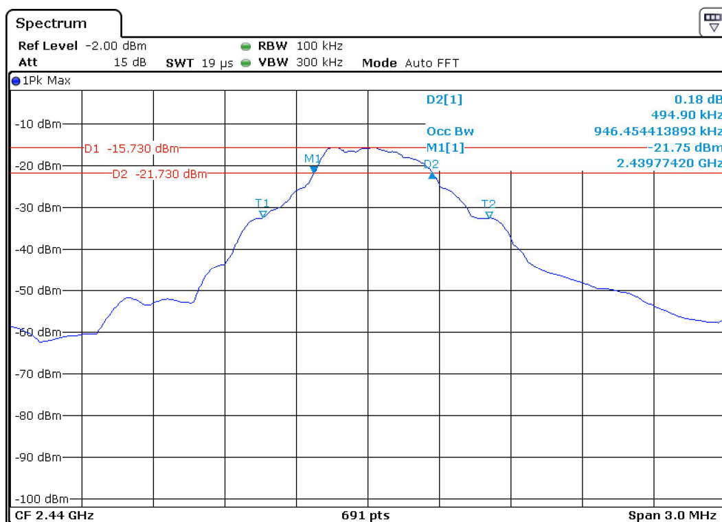
Mid Channel – Bandwidth 0.947MHz
