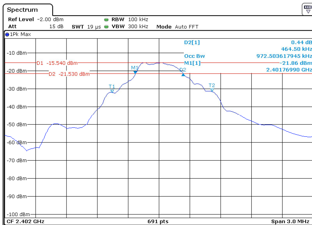
Low Channel – Bandwidth 0.973MHz
