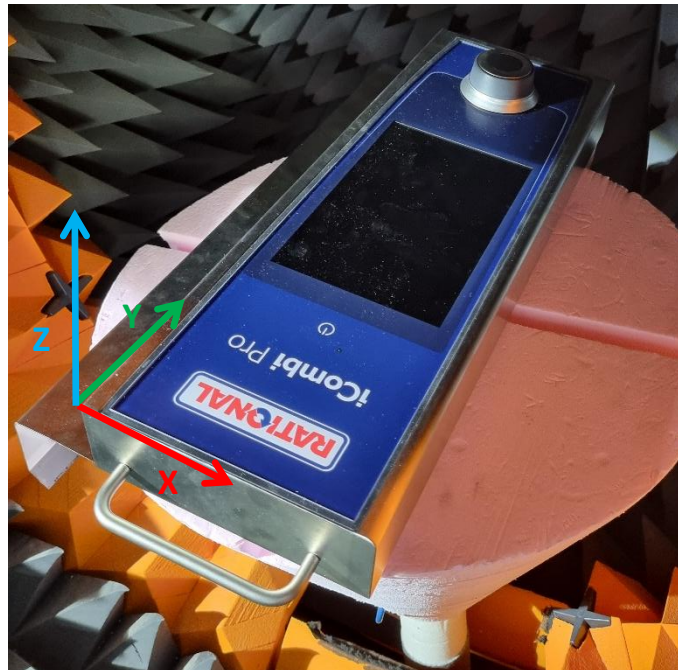
Chamber Setup of device 2
