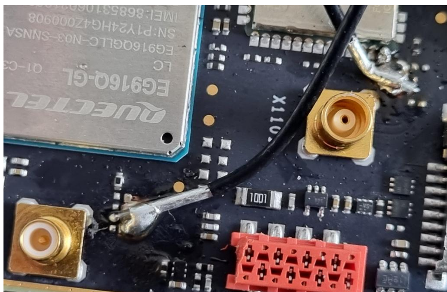
Cables soldered to board
