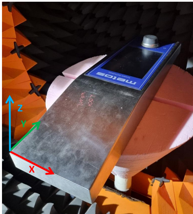
Chamber Setup of device 3
