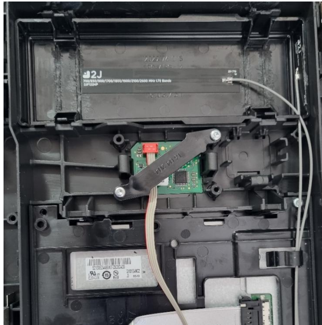
Antenna mounting in device 1
