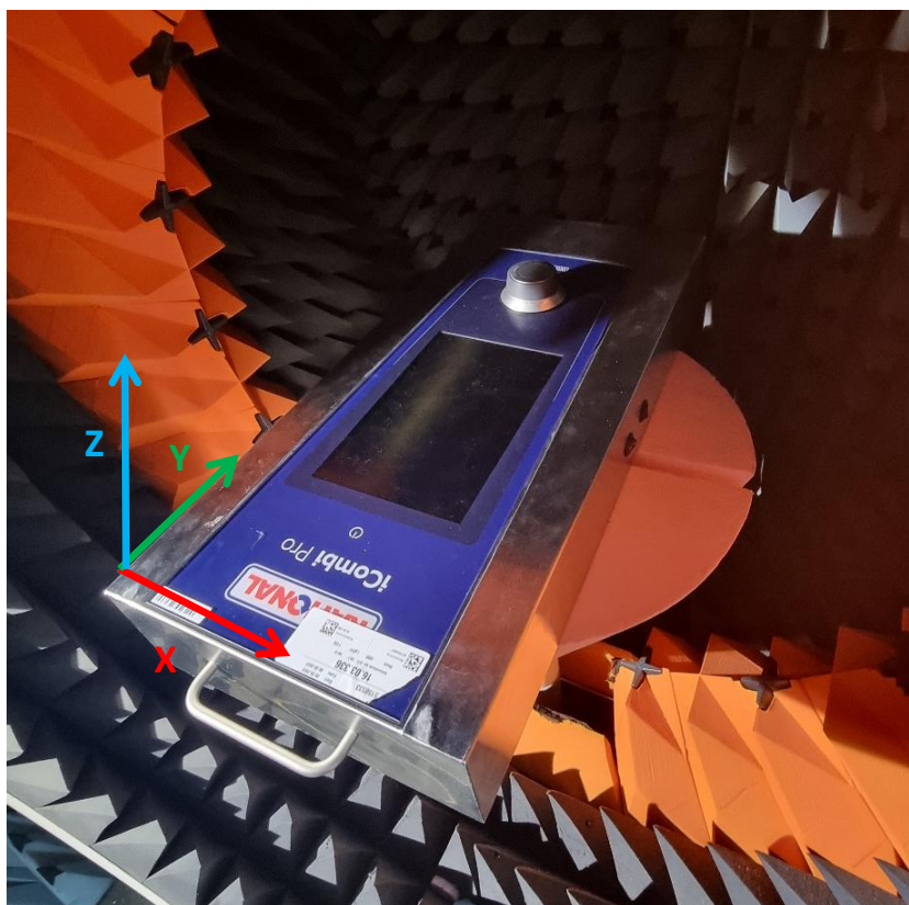
Chamber Setup of device 1
