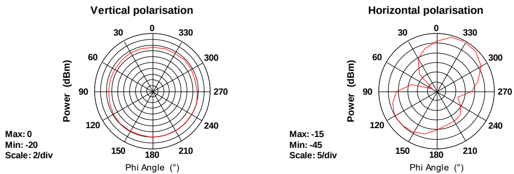
Fig. 5: Test results vertical and horizontal polarization pattern 2437 MHz
