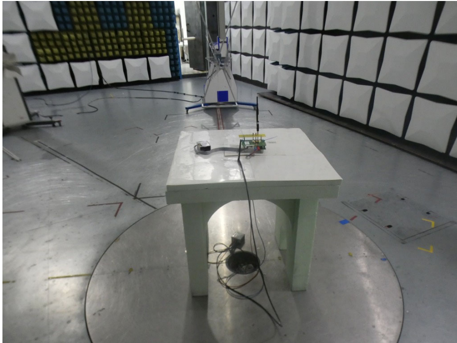
Photo 3: Test setup for radiated measurements below 1 GHz
