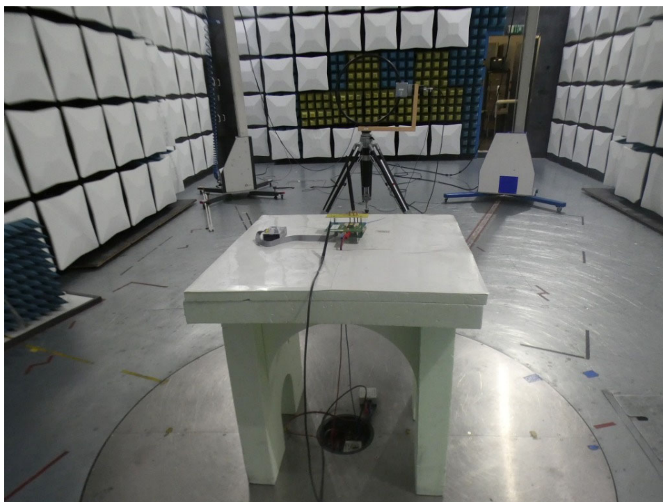
Photo 2: Test setup for radiated measurements below 30 MHz
