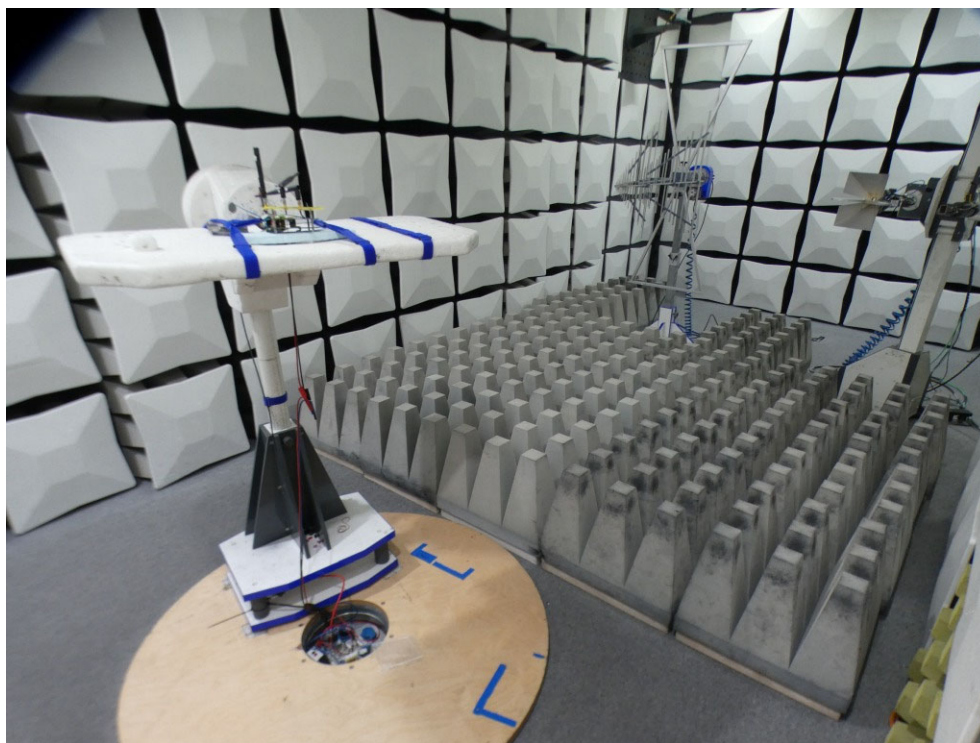
Photo 4: Test setup for radiated measurements above 1 GHz
