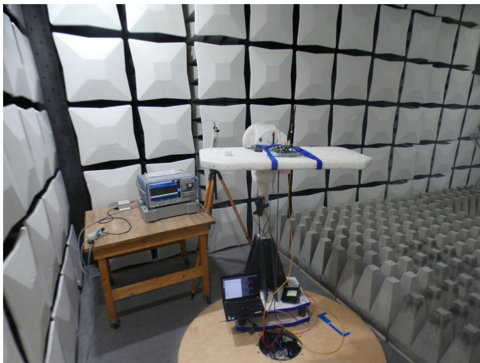
Photo 7: Test setup for radiated measurements above 26 GHz
