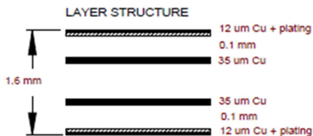
Figure 12. Reference PCB stack-up.
