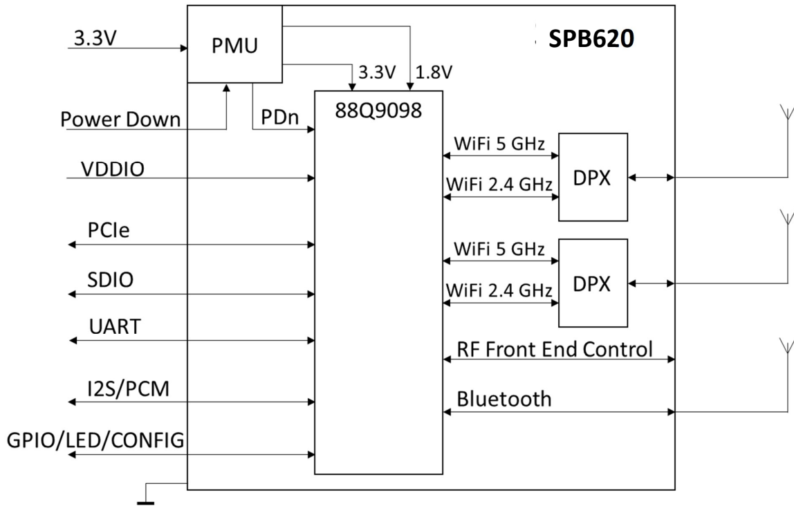
Figure 1. Block diagram.
