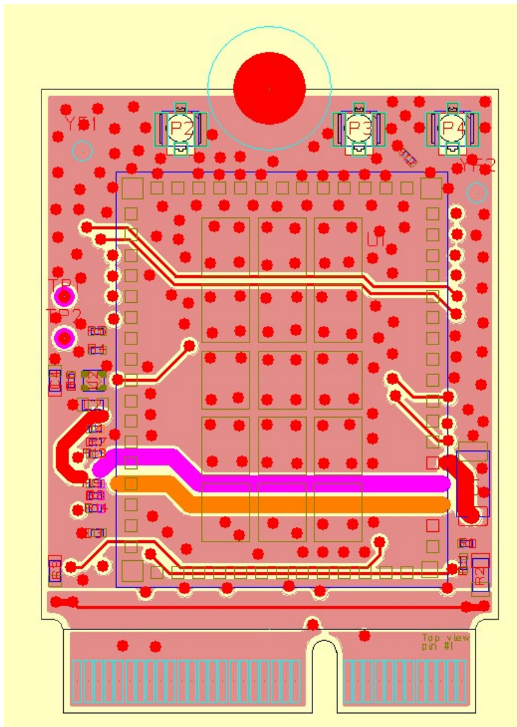
Figure 7. Third layer (ground, signals and supply).
