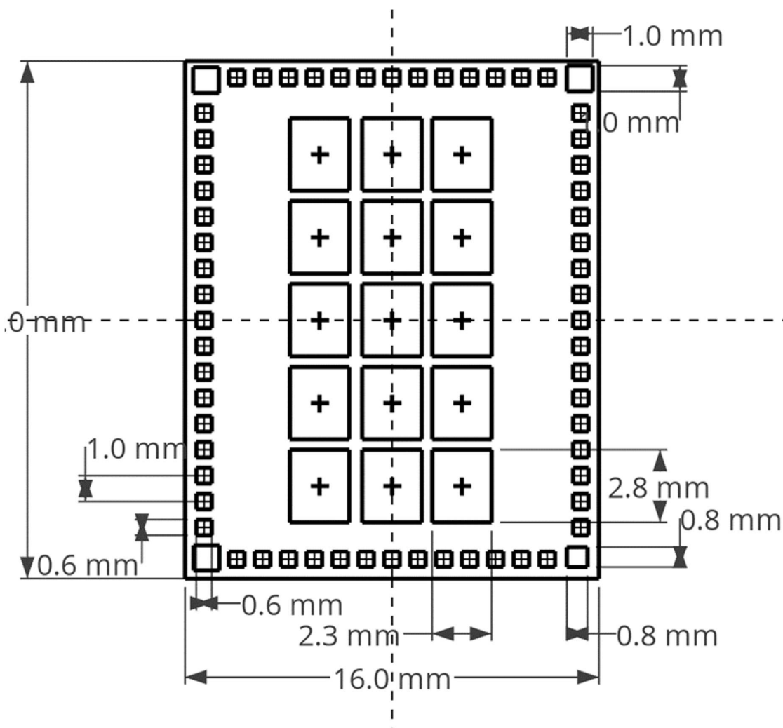
Figure 11. Recommended land pattern on the PCB, top view.
