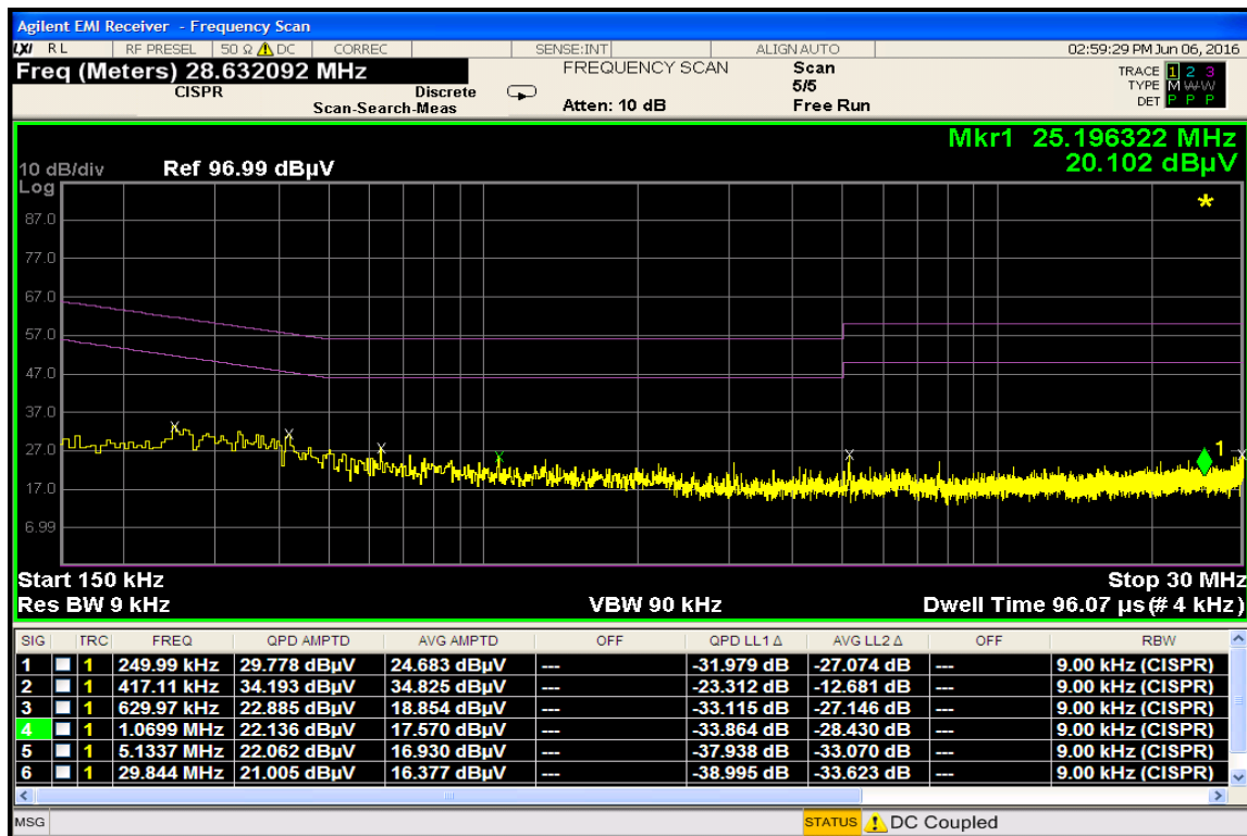
Plot 7-55. Line-Conducted Test Plot (N)
