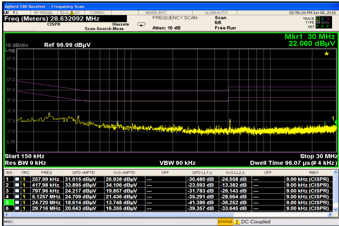
Plot 7-54. Line-Conducted Test Plot (L1)
