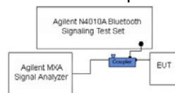
Figure 7-2. Test Instrument & Measurement Setup
