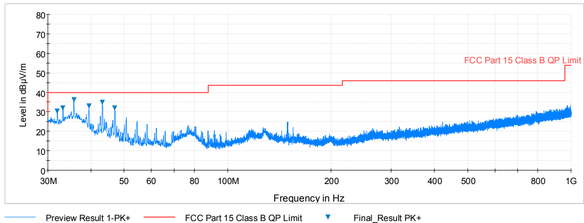
Plot 7-27. Radiated Spurious Plot below 1GHz (802.11a – U3 Ch. 157, Ant. Pol. V)
