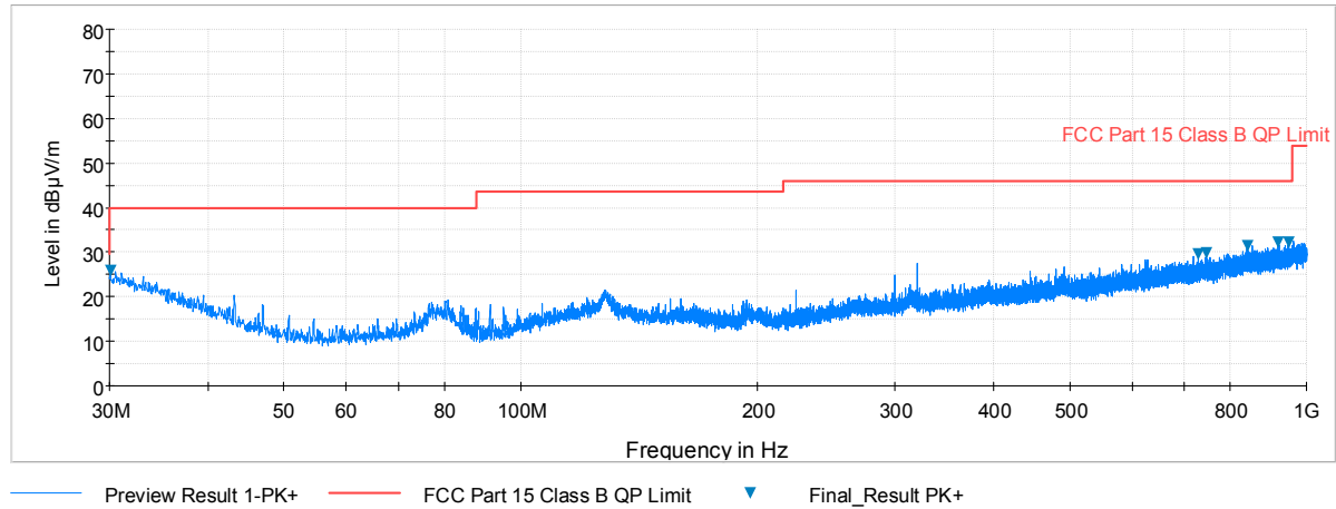
Plot 7-26. Radiated Spurious Plot below 1GHz (802.11a – U3 Ch. 157, Ant. Pol. H)
