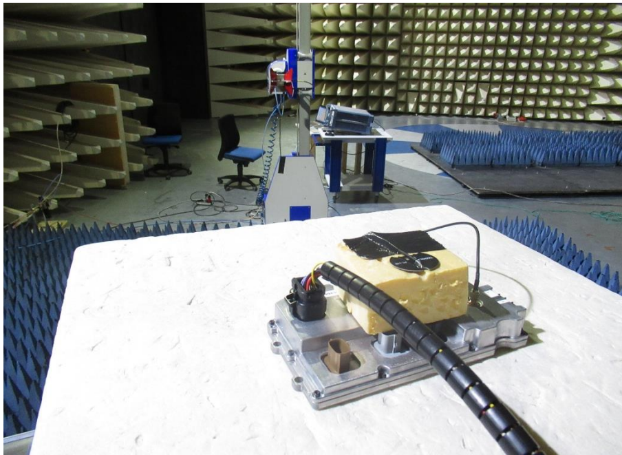
Anechoic chamber
