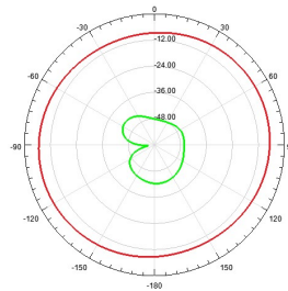
Y-Z Plane
