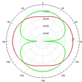
X-Z Plane
