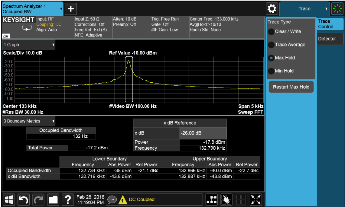
Figure 2 - Emission Bandwidth
