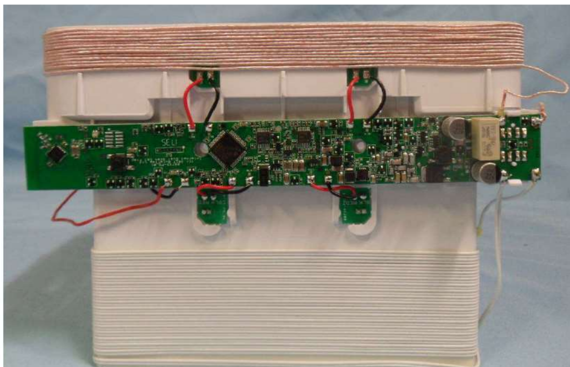
Internal view - Frame and Tunnel (Cover and battery compartment removed)
