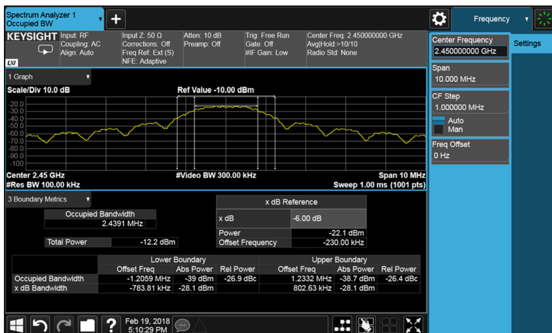
Figure 2 - 2450 MHz – 6 dB Bandwidth and 99% Occupied Bandwidth
