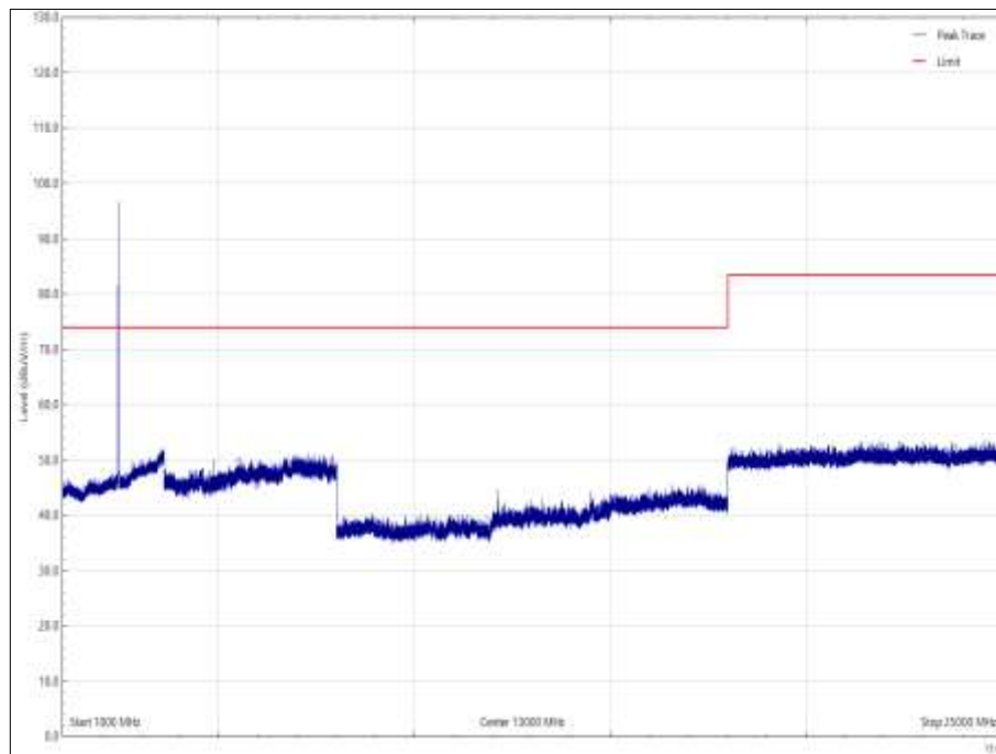
Figure 13 - 2425 MHz, 1 GHz to 25 GHz, Vertical, X Orientation: - Peak
