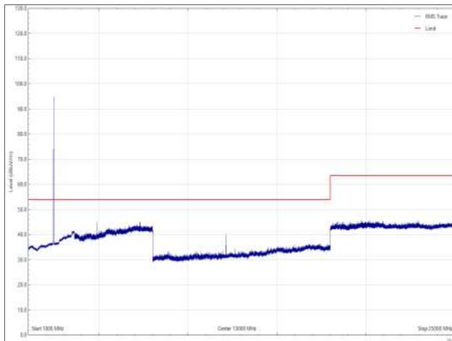
Figure 14 - 2425 MHz, 1 GHz to 25 GHz, Vertical, X Orientation: - Average
