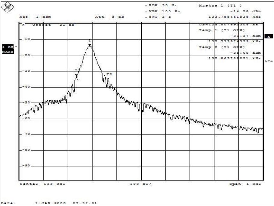
Figure 2 - Emission Bandwidth
