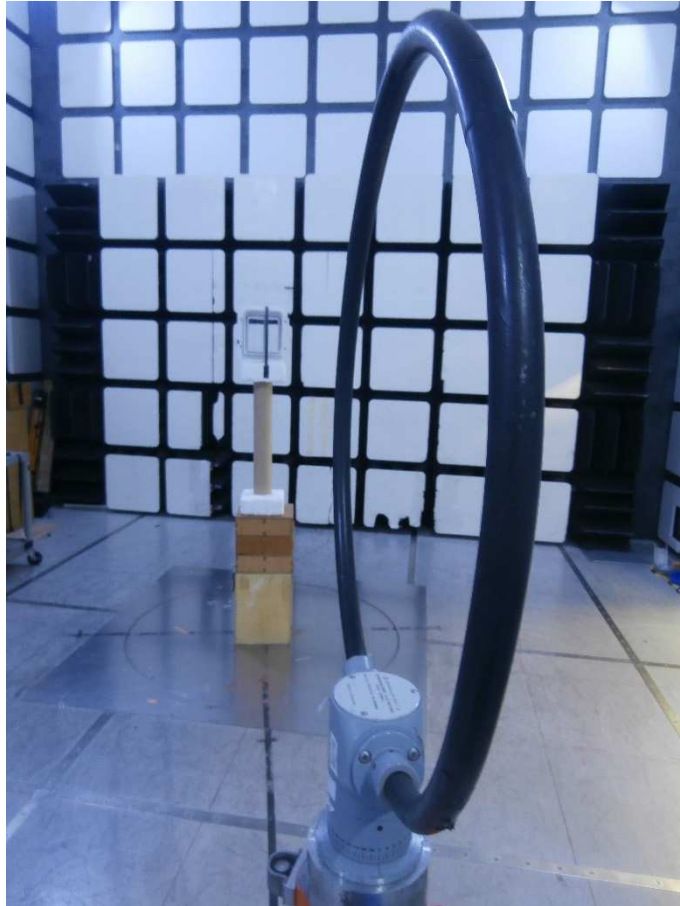
Radiated Emissions < 30 MHz (Chamber)
