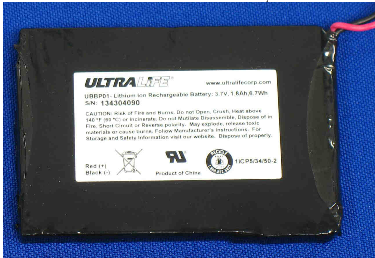
Figure 5: Battery Pack
