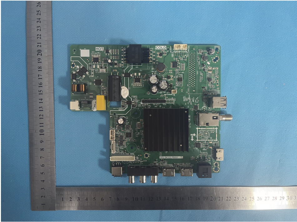
Solder Board-Component View 8
