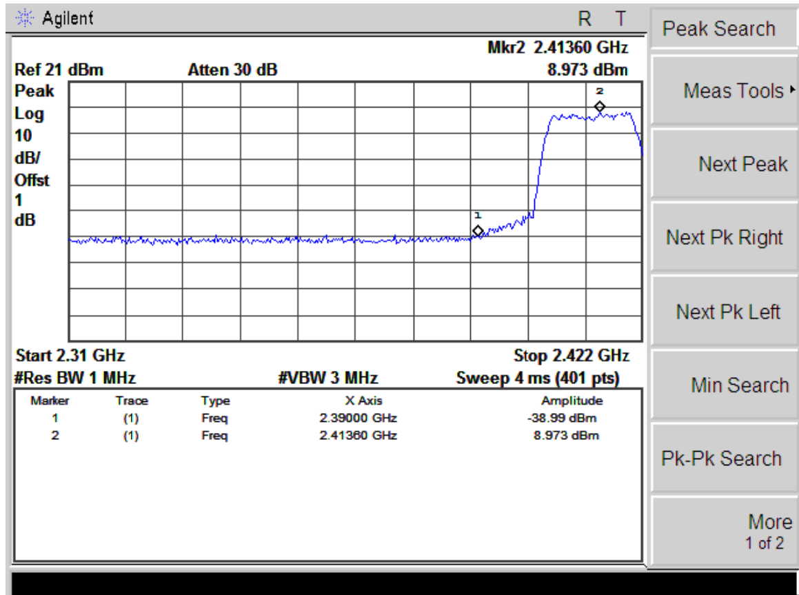
(Plot 4.5.2 A1: Channel 1: 2412MHz @ 802.11g)
