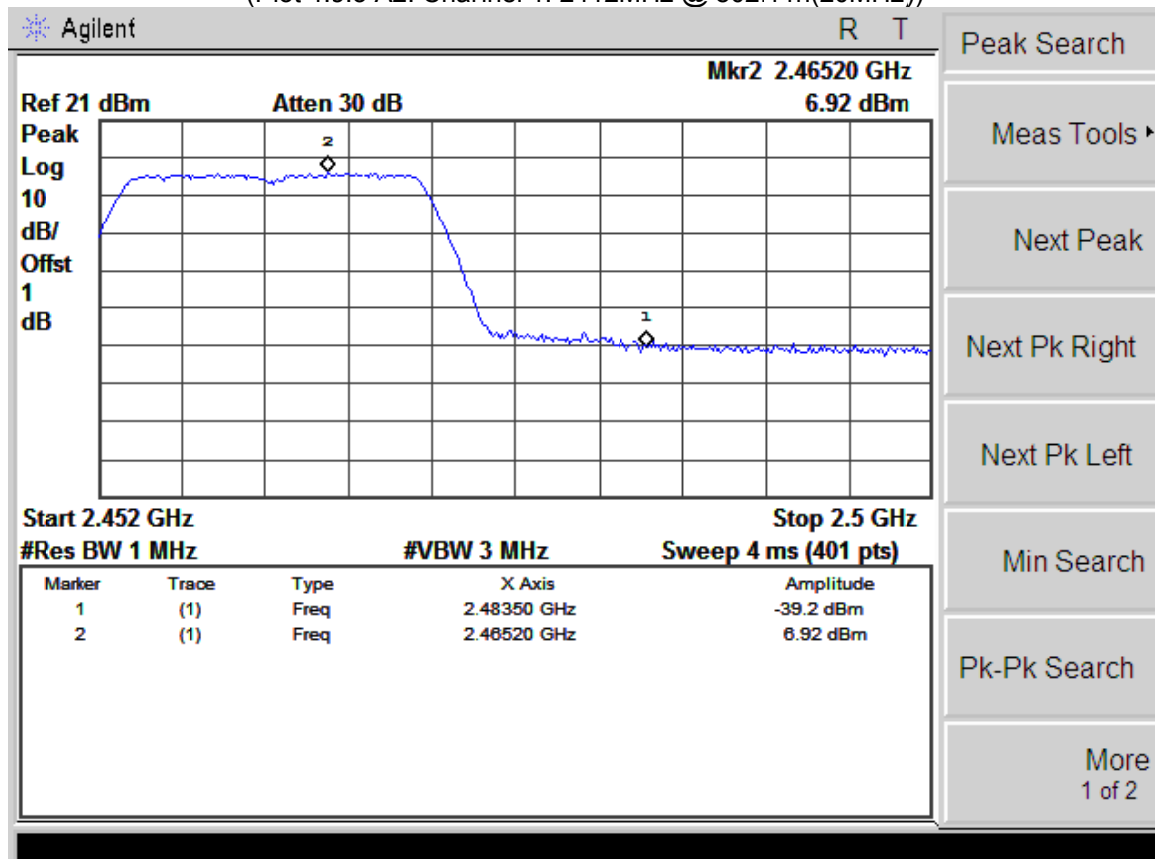
(Plot 4.5.3 A3: Channel 11: 2462MHz @ 802.11n(20MHz))
