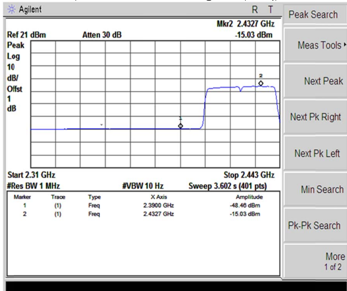
(Plot 4.5.3 A2: Channel 3: 2422MHz @ 802.11n(40MHz))
