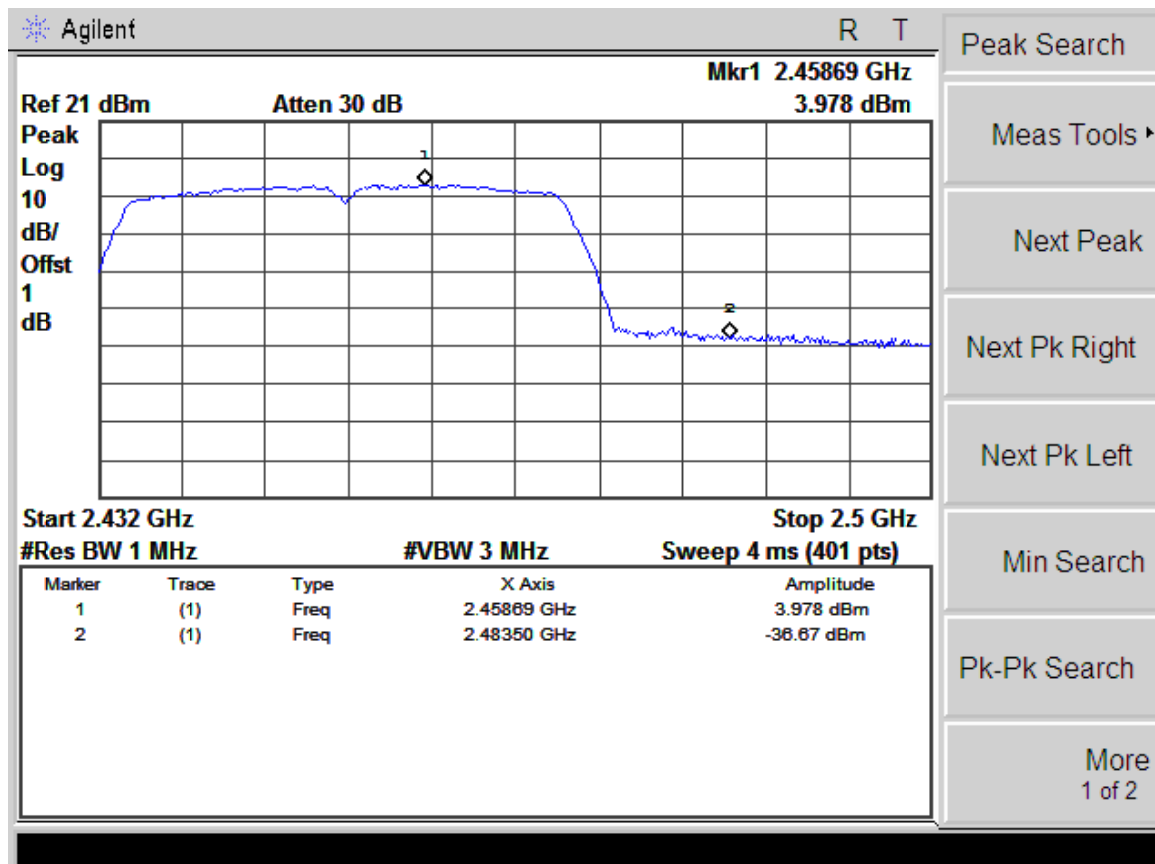
(Plot 4.5.3 A3: Channel 9: 2452MHz @ 802.11n(40MHz))
