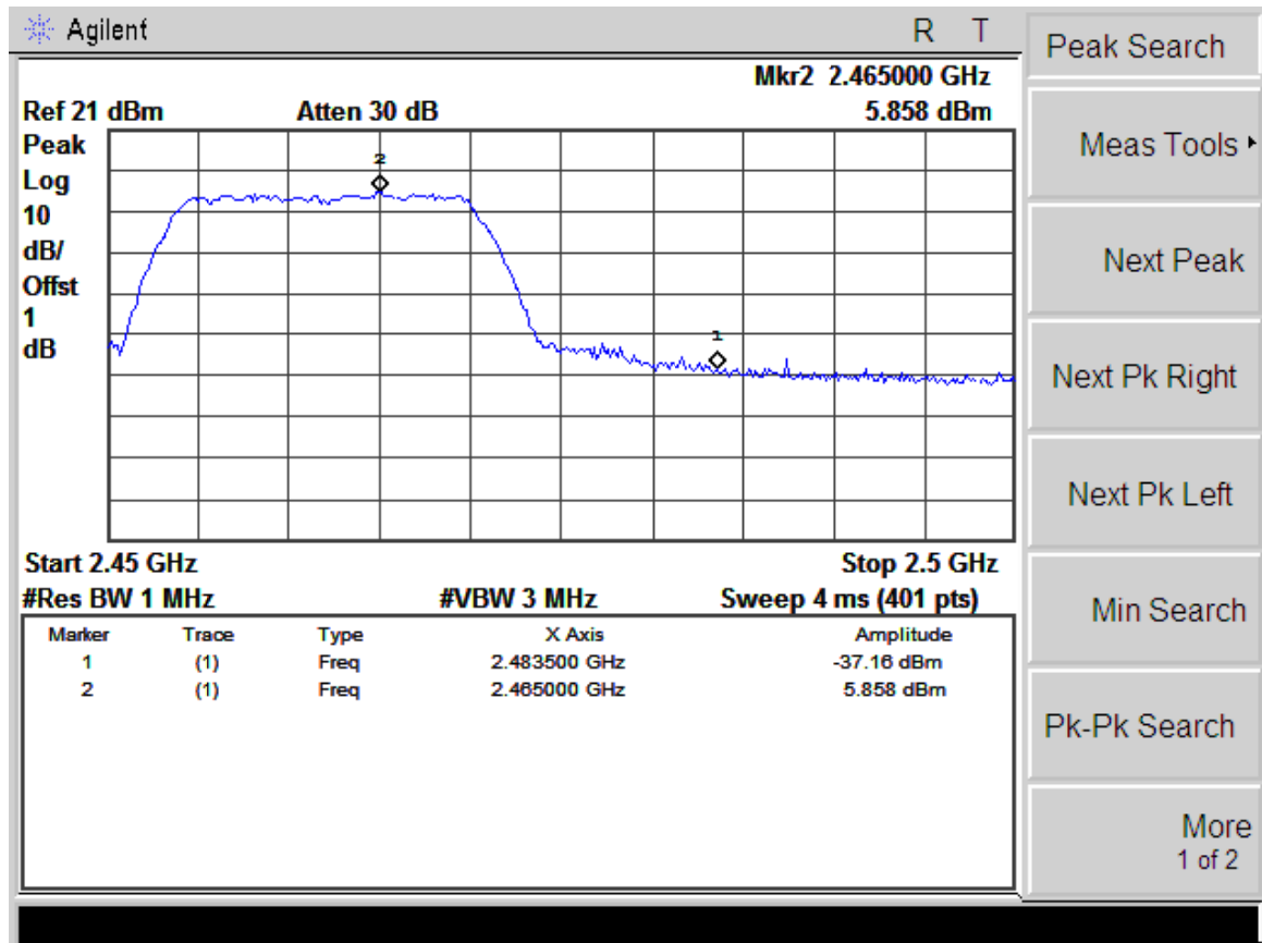
(Plot 4.5.2 A3: Channel 11: 2462MHz @ 802.11g)
