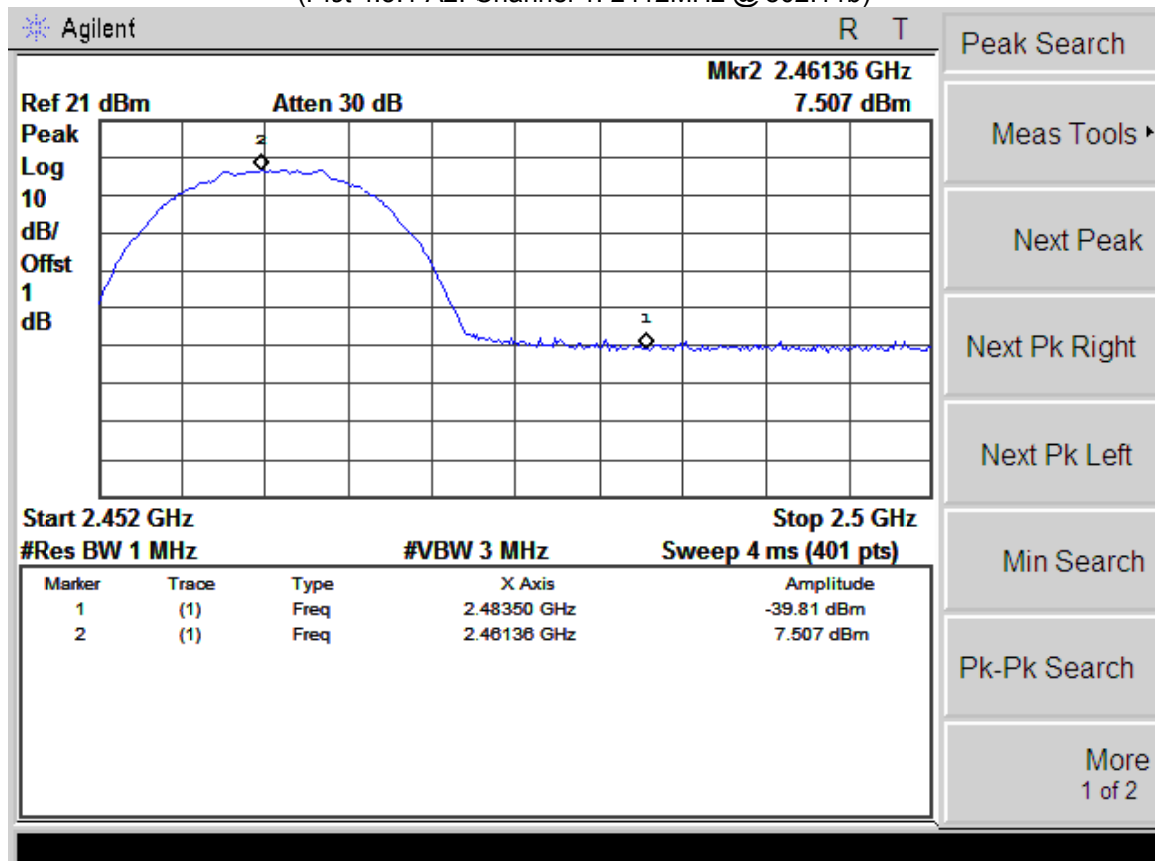
(Plot 4.5.1 A3: Channel 11: 2462MHz @ 802.11b)
