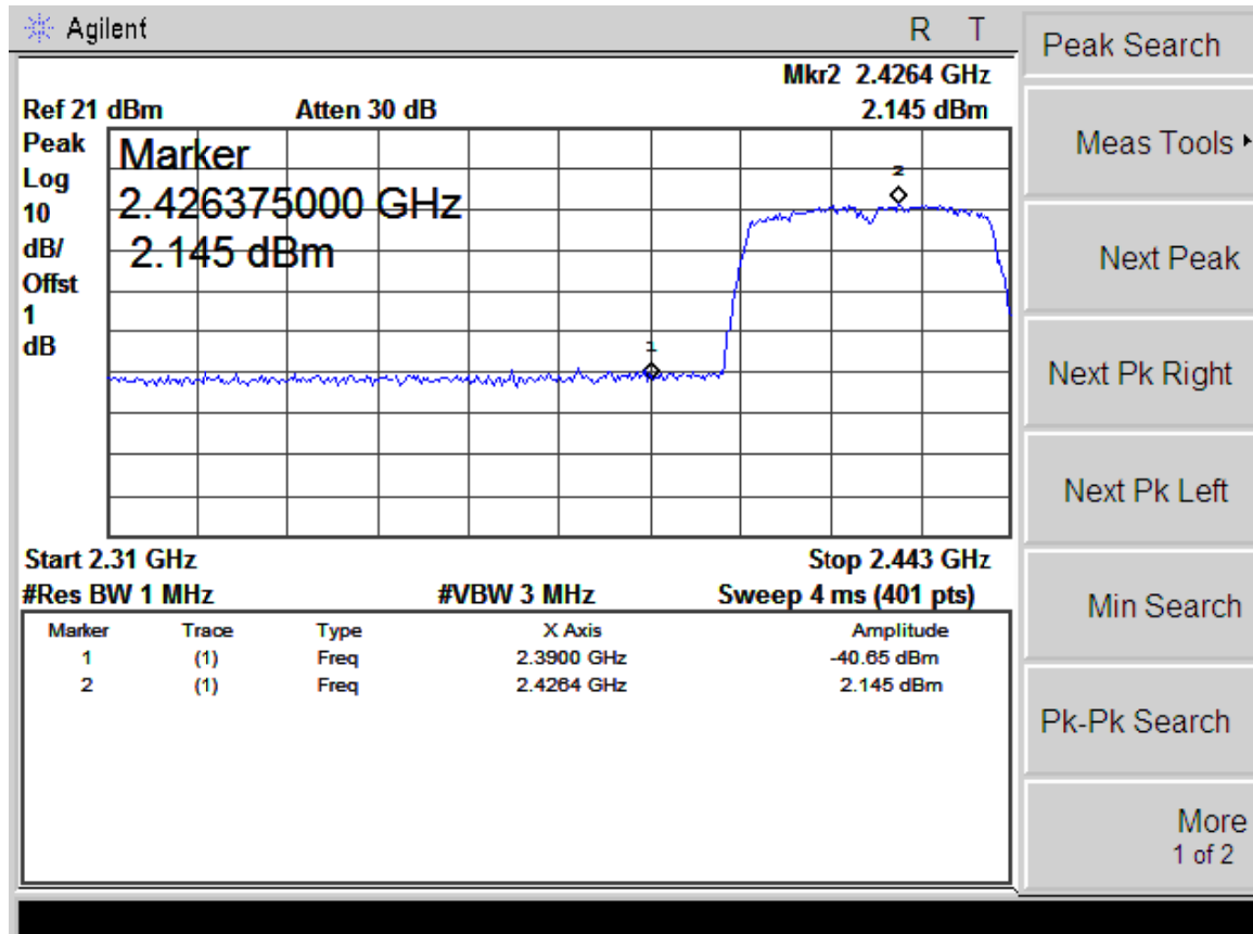
(Plot 4.5.3 A1: Channel 3: 2422MHz @ 802.11n(40MHz))
