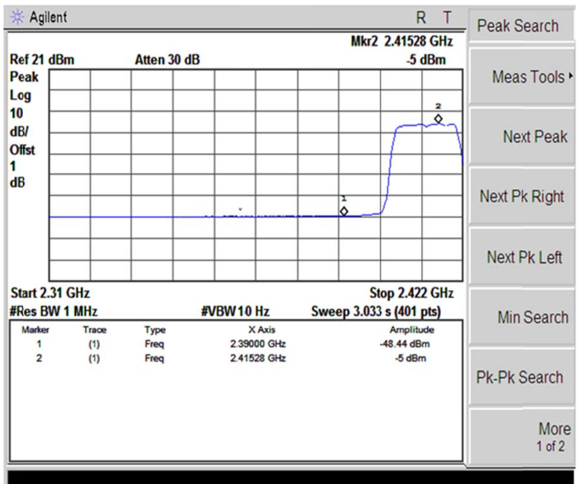
(Plot 4.5.2 A2: Channel 1: 2412MHz @ 802.11g)
