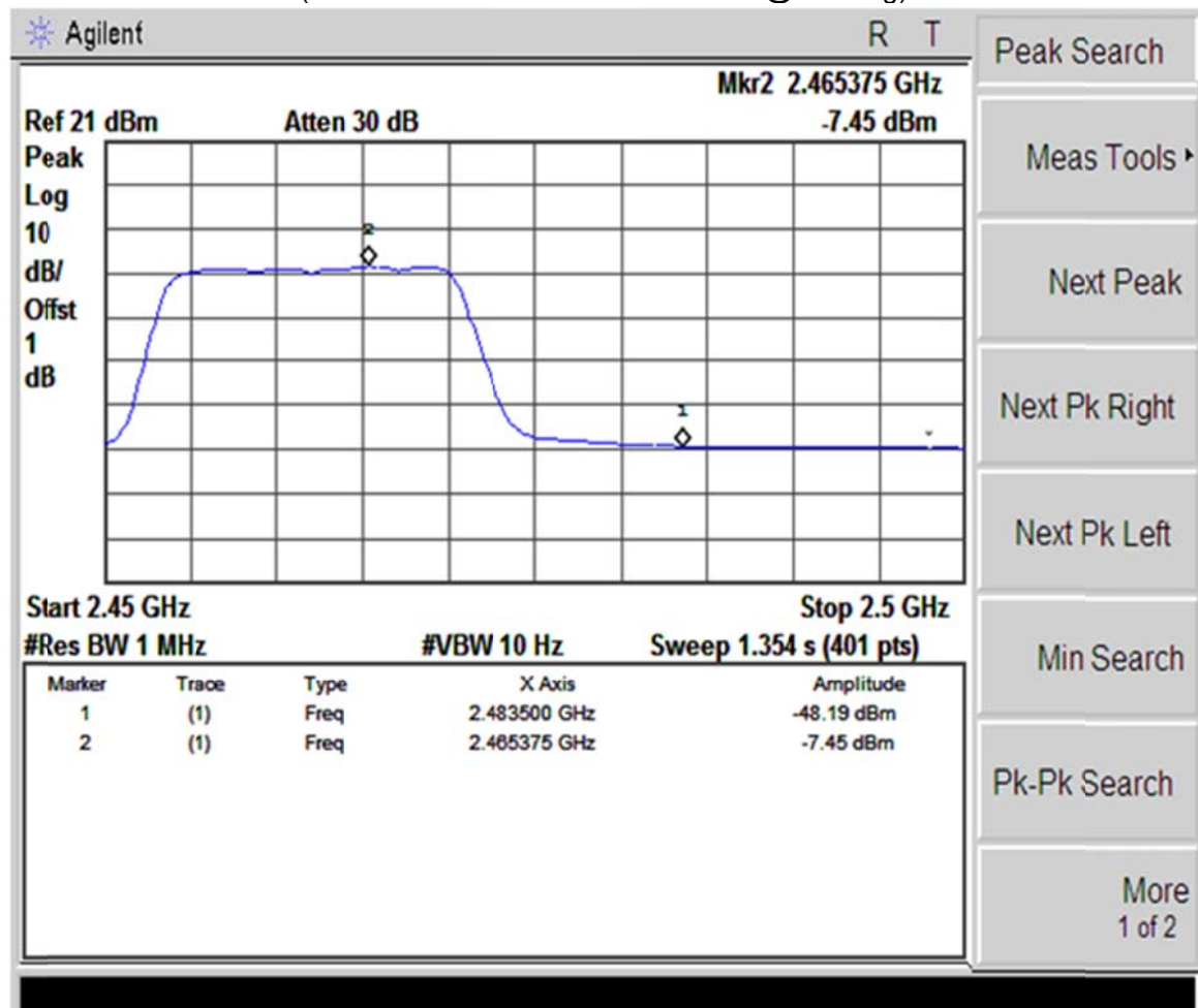
(Plot 4.5.2 A3: Channel 11: 2462MHz @ 802.11g)
