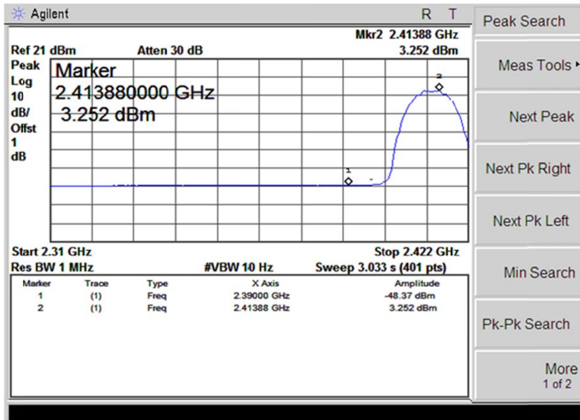
(Plot 4.5.1 A2: Channel 1: 2412MHz @ 802.11b)
