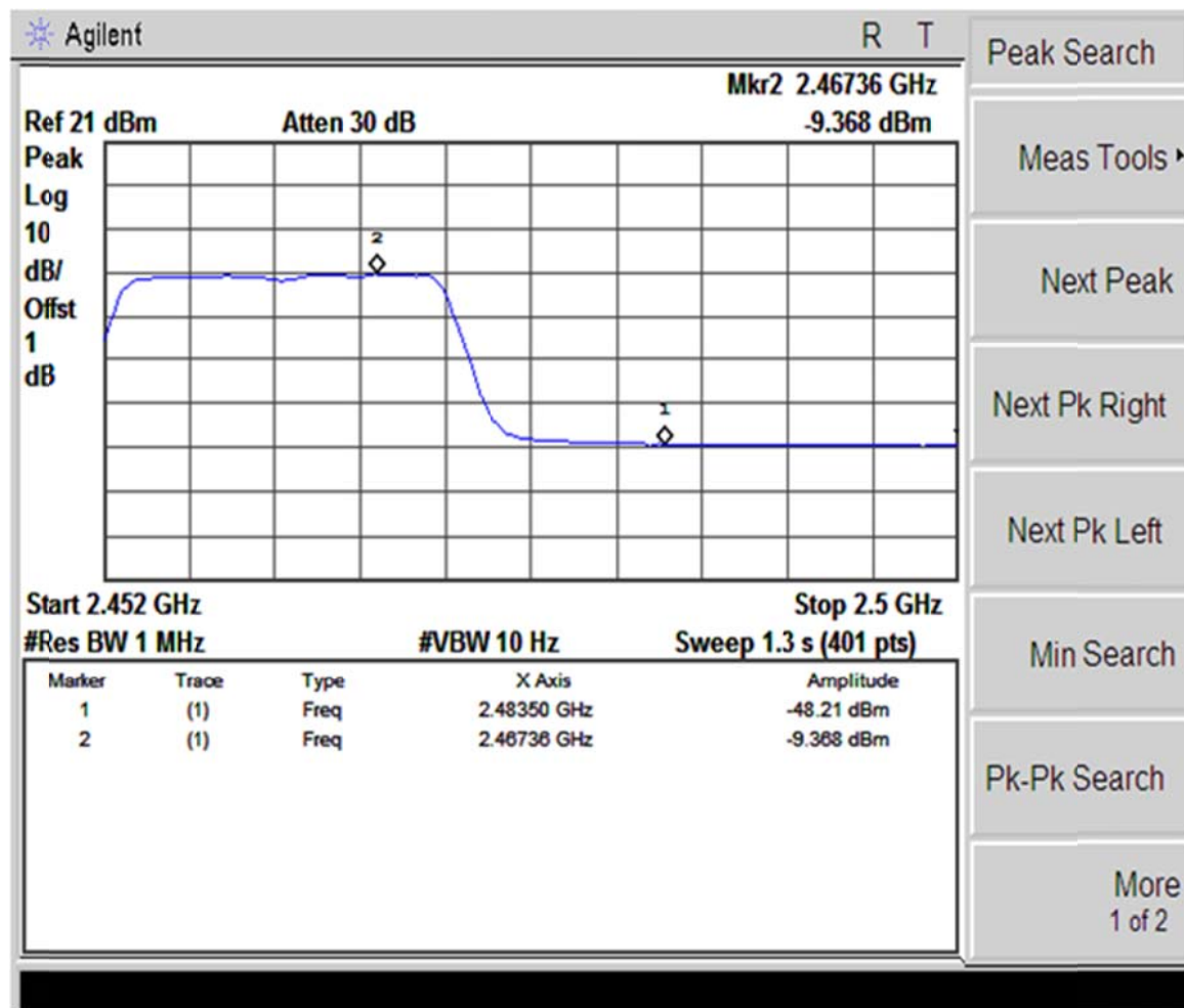
(Plot 4.5.3 A4: Channel 11: 2462MHz @ 802.11n(20MHz))
