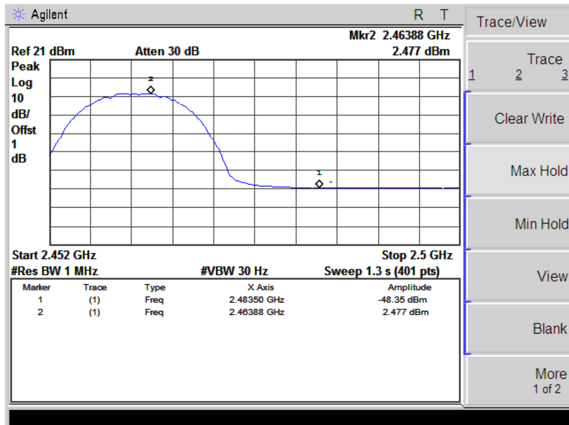
(Plot 4.5.1 A4: Channel 11: 2462MHz @ 802.11b)
