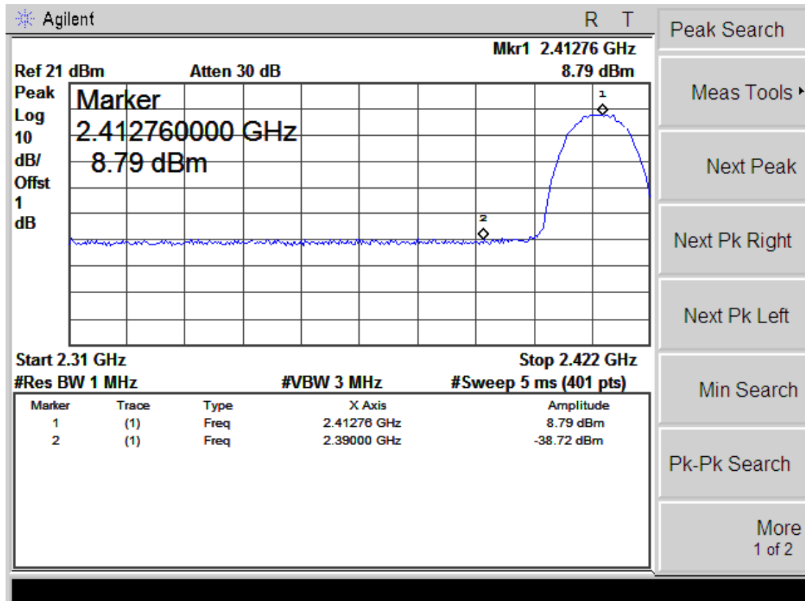
(Plot 4.5.1 A1: Channel 1: 2412MHz @ 802.11b)
