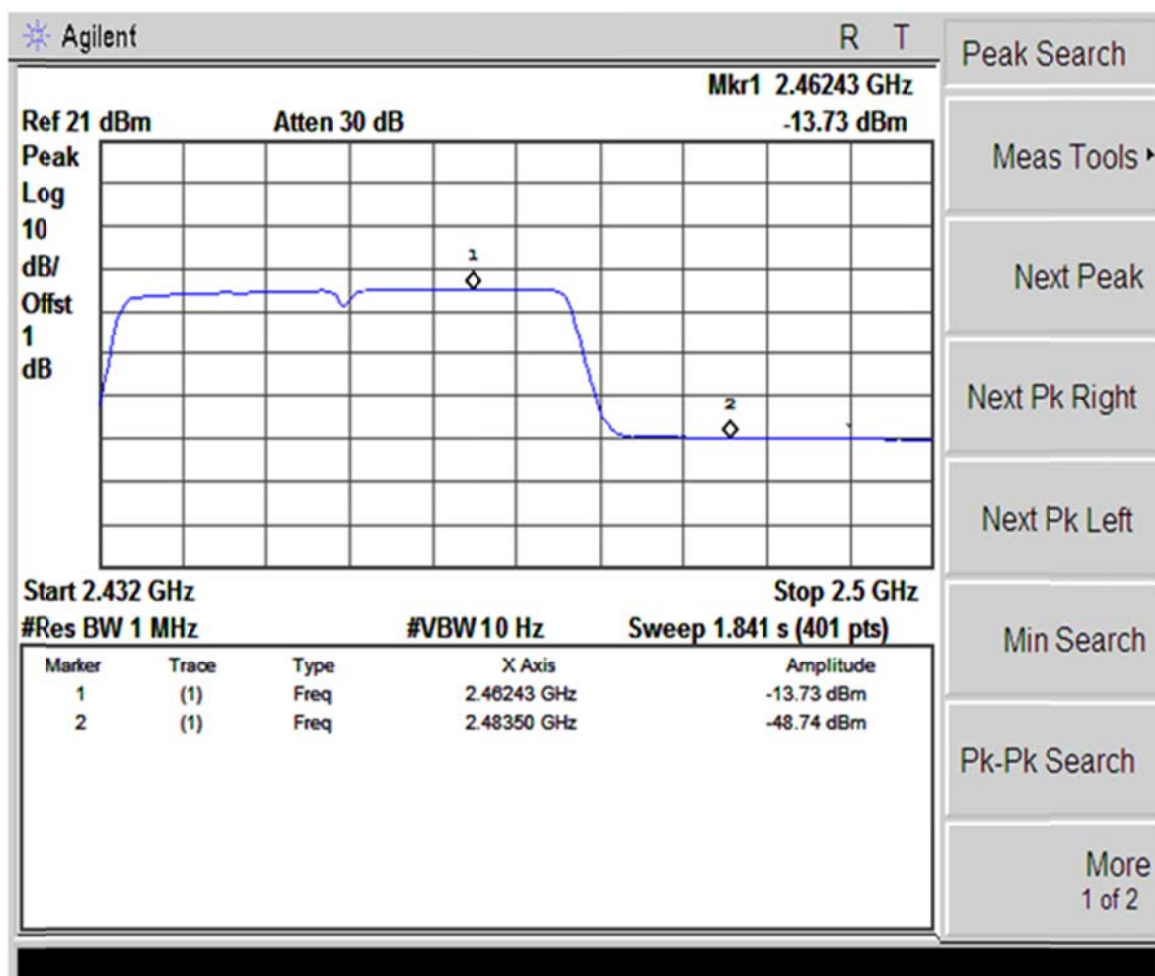
(Plot 4.5.3 A4: Channel 9: 2452MHz @ 802.11n(40MHz))
