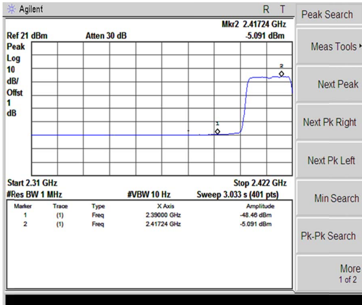
(Plot 4.5.3 A2: Channel 1: 2412MHz @ 802.11n(20MHz))
