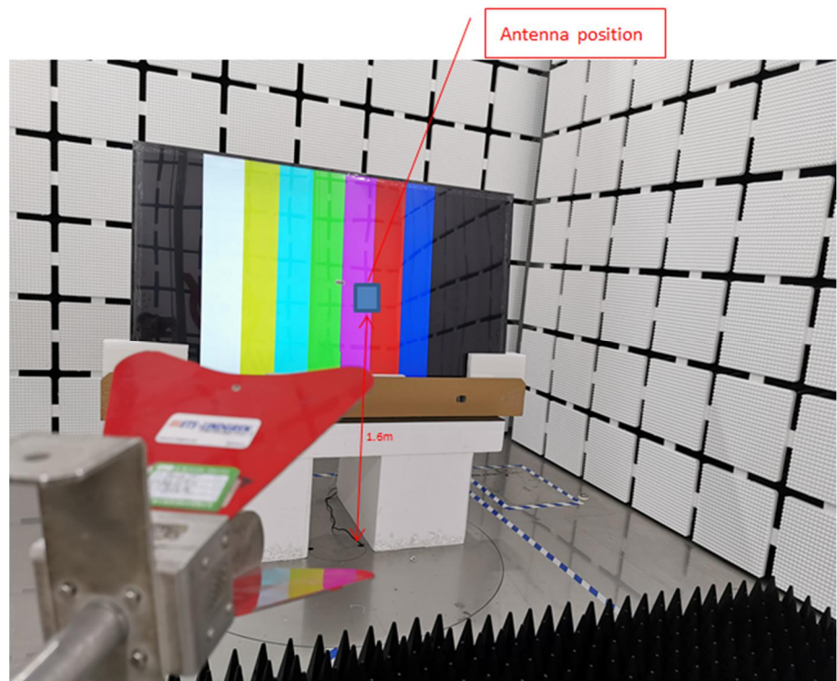
Radiation Emission Test Setup (1GHz to 18GHz)
