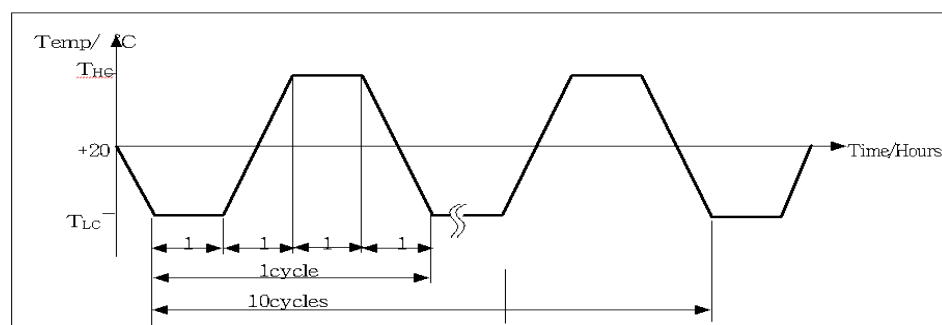
Figure5. Temperature Cycling
