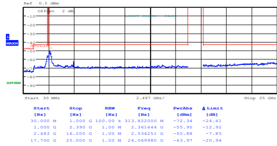
Figure 8.3-32: Conducted spurious emissions within restricted bands for 802.11n HT20, MCS 0, high channel
