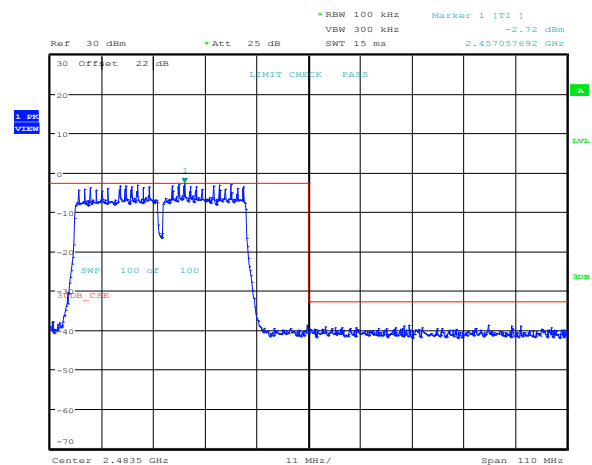
Figure 8.3-54: Band edge emission outside restricted bands at 2.4835 GHz for 802.11g, 6 Mbps
