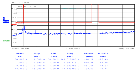
Figure 8.3-36: Conducted spurious emissions within restricted bands for 802.11n HT20, MCS 7, low channel
