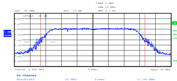
Figure 8.2-2: Output power on 802.11g, sample plot
