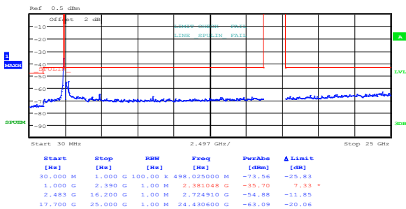
Figure 8.3-26: Conducted spurious emissions within restricted bands for 802.11n HT40, MCS 0, low channel
