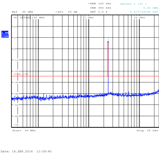
Figure 8.3-19: Conducted spurious emissions outside restricted bands for 802.11b, 11 Mbps, high channel
