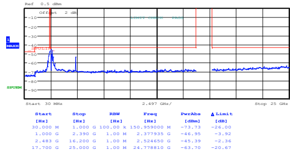
Figure 8.3-34: Conducted spurious emissions within restricted bands for 802.11b, 11 Mbps, low channel
