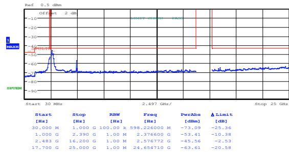
Figure 8.3-30: Conducted spurious emissions within restricted bands for 802.11b, 1 Mbps, high channel
