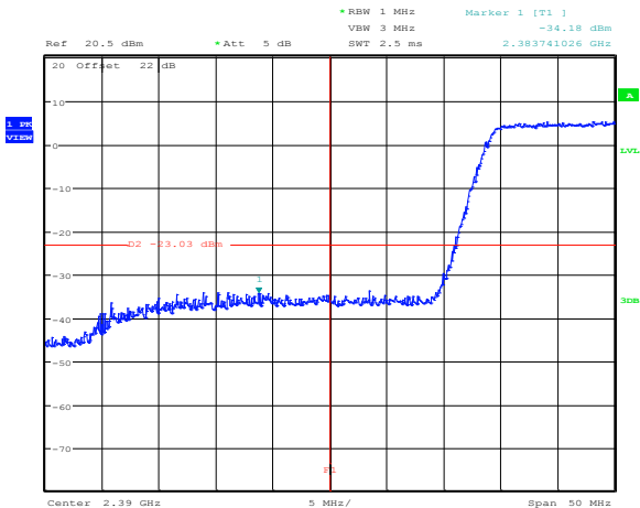
Figure 8.3-65: Band edge emission within restricted bands at 2.4 GHz for 802.11n HT20, MCS 0, peak
