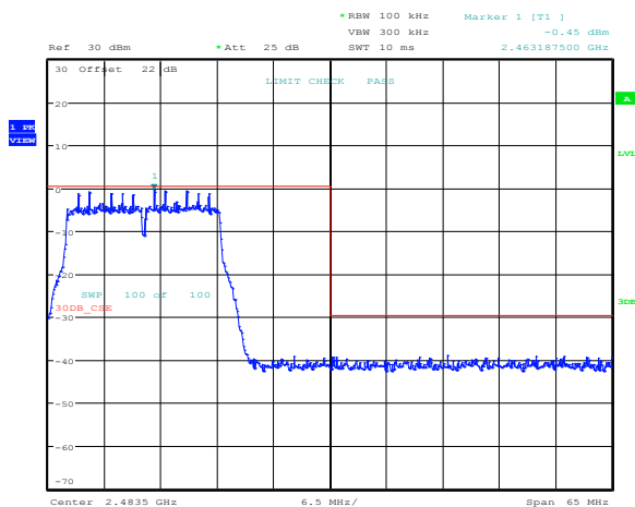
Figure 8.3-53: Band edge emission outside restricted bands at 2.4835 GHz for 802.11b, 1 Mbps
