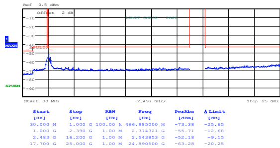
Figure 8.3-29: Conducted spurious emissions within restricted bands for 802.11n HT20, MCS 0, mid channel
