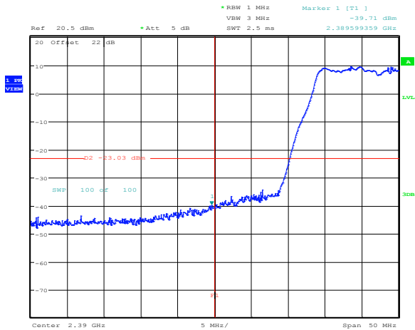
Figure 8.3-69: Band edge emission within restricted bands at 2.4 GHz for 802.11b, 11 Mbps, peak
