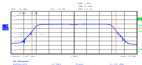
Figure 8.2-3: Output power on 802.11n HT20, sample plot
