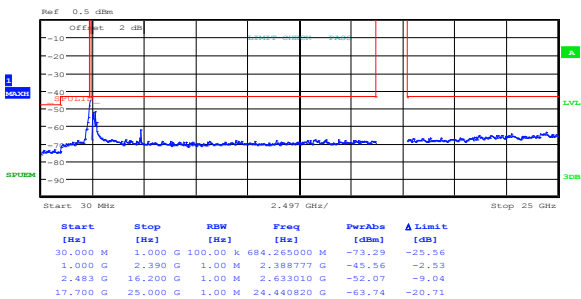
Figure 8.3-25: Conducted spurious emissions within restricted bands for 802.11n HT20, MCS 0, low channel
