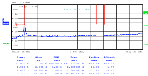
Figure 8.3-35: Conducted spurious emissions within restricted bands for 802.11g, 54 Mbps, low channel
