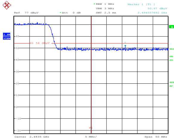
Figure 8.3-98: Cabinet radiation at the restricted band edge at 2.4835 GHz for 802.11n HT20
