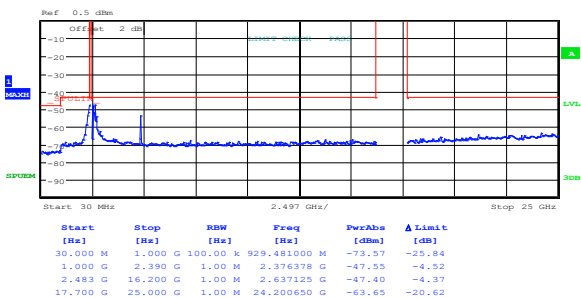
Figure 8.3-23: Conducted spurious emissions within restricted bands for 802.11b, 1 Mbps, low channel
