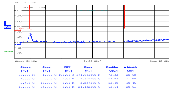
Figure 8.3-40: Conducted spurious emissions within restricted bands for 802.11n HT20, MCS 7, mid channel
