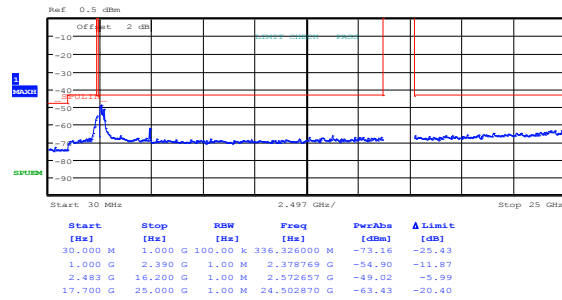
Figure 8.3-42: Conducted spurious emissions within restricted bands for 802.11g, 54 Mbps, high channel
