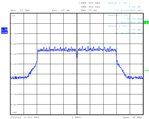
Figure 8.1-1: 6 dB bandwidth on 802.11b, sample plot
