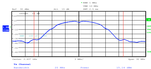
Figure 8.2-1: Output power on 802.11b, sample plot
