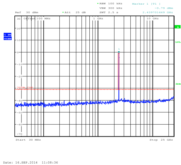
Figure 8.3-18: Conducted spurious emissions outside restricted bands for 802.11n HT20, MCS 7, mid channel
