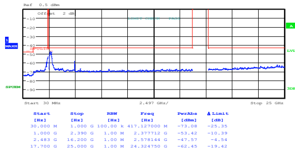
Figure 8.3-41: Conducted spurious emissions within restricted bands for 802.11b, 11 Mbps, high channel
