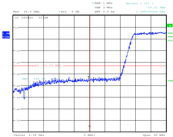
Figure 8.3-73: Band edge emission within restricted bands at 2.4 GHz for 802.11n HT20, MCS 7, peak
