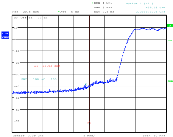
Figure 8.3-61: Band edge emission within restricted bands at 2.4 GHz for 802.11b, 1 Mbps, peak
