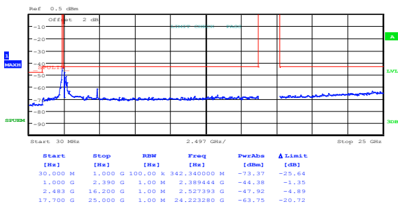
Figure 8.3-24: Conducted spurious emissions within restricted bands for 802.11g, 6 Mbps, low channel
