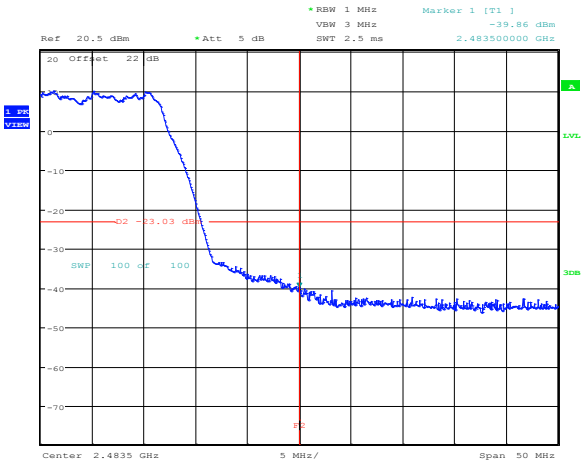
Figure 8.3-85: Band edge emission within restricted bands at 2.4835 GHz for 802.11b, 11 Mbps, peak
