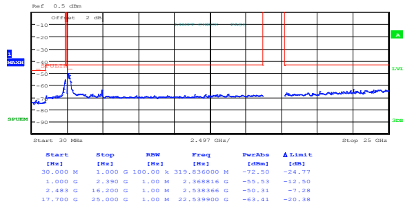
Figure 8.3-43: Conducted spurious emissions within restricted bands for 802.11n HT20, MCS 7, high channel
