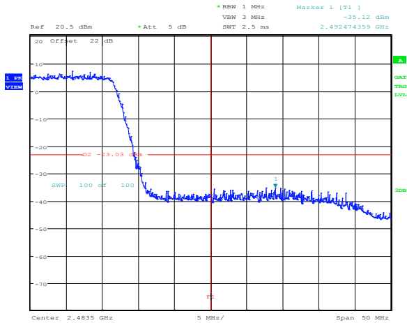
Figure 8.3-89: Band edge emission within restricted bands at 2.4835 GHz for 802.11n HT20, MCS 7, peak
