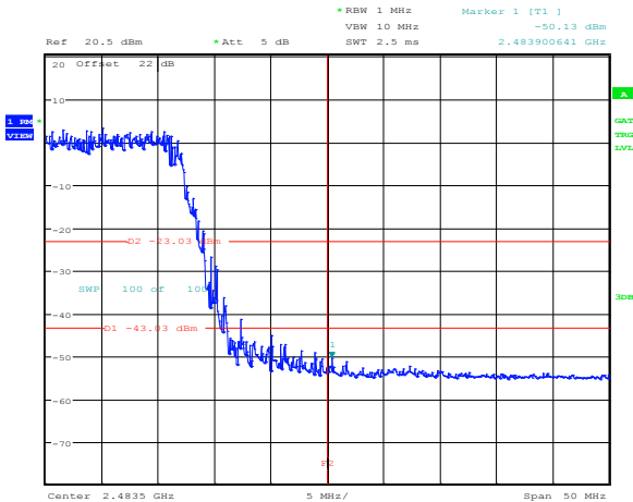
Figure 8.3-86: Band edge emission within restricted bands at 2.4835 GHz for 802.11b, 11 Mbps, average
