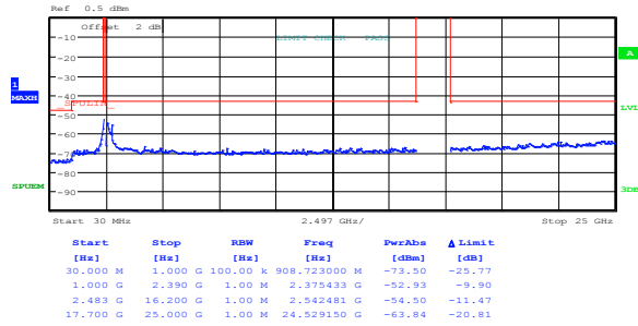
Figure 8.3-33: Conducted spurious emissions within restricted bands for 802.11n HT40, MCS 0, high channel
