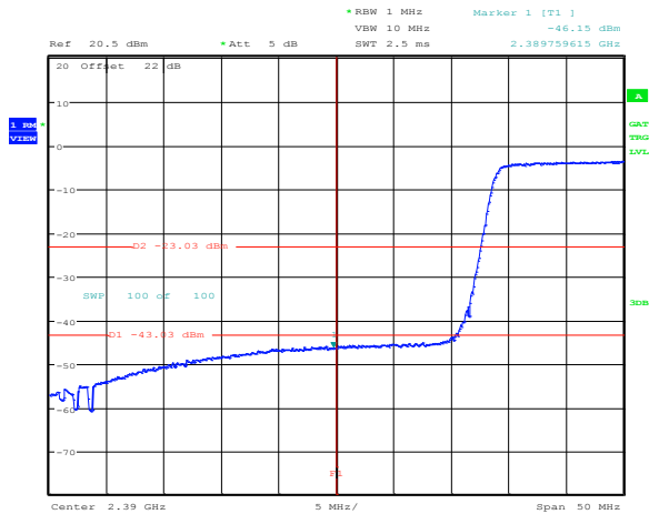
Figure 8.3-74: Band edge emission within restricted bands at 2.4 GHz for 802.11n HT20, MCS 7, average
