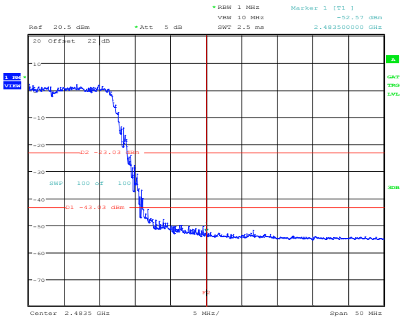
Figure 8.3-78: Band edge emission within restricted bands at 2.4835 GHz for 802.11b, 1 Mbps, average
