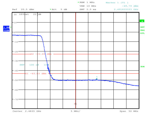
Figure 8.3-90: Band edge emission within restricted bands at 2.4835 GHz for 802.11n HT20, MCS 7, average
