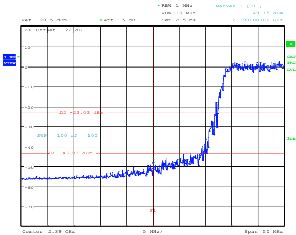
Figure 8.3-70: Band edge emission within restricted bands at 2.4 GHz for 802.11b, 11 Mbps, average
