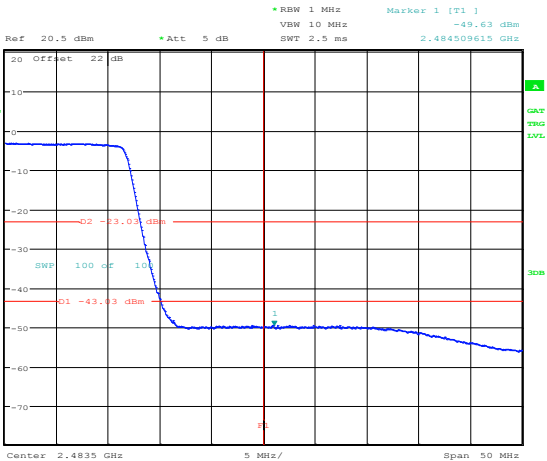
Figure 8.3-82: Band edge emission within restricted bands at 2.4835 GHz for 802.11n HT20, MCS 0, average
