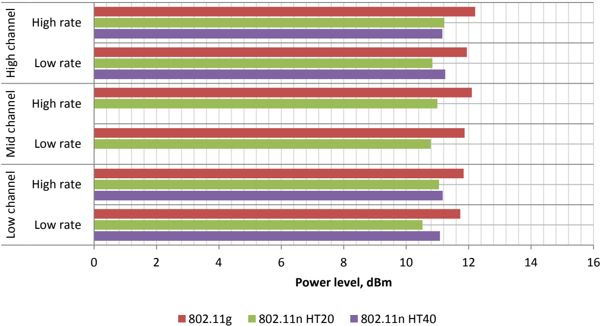
Figure 8.2-5: Output power comparison
