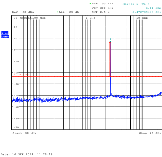
Figure 8.3-8: Conducted spurious emissions outside restricted bands for 802.11b, 1 Mbps, high channel
