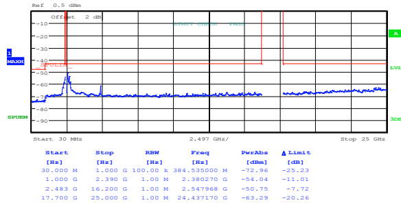
Figure 8.3-39: Conducted spurious emissions within restricted bands for 802.11g, 54 Mbps, mid channel
