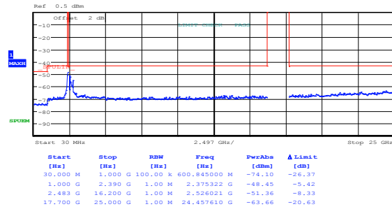
Figure 8.3-44: Conducted spurious emissions within restricted bands for 802.11n HT40, MCS 7, high channel
