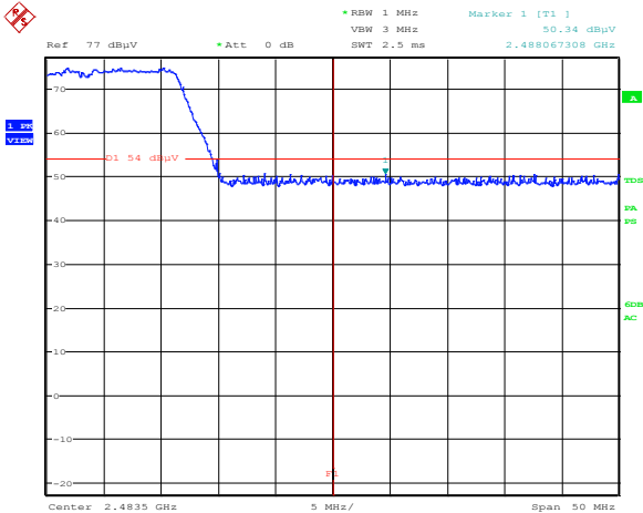
Figure 8.3-94: Cabinet radiation at the restricted band edge at 2.4835 GHz for 802.11b
