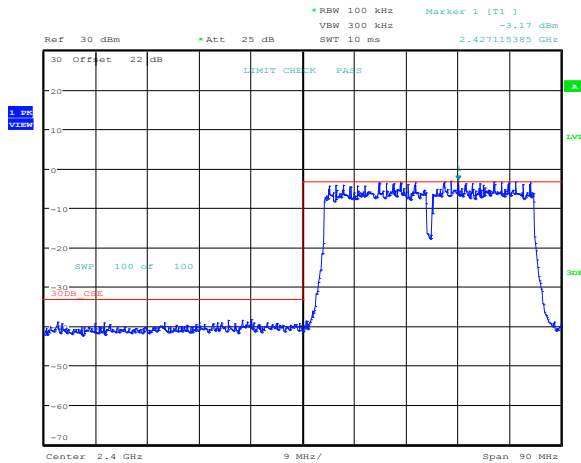
Figure 8.3-50: Band edge emission outside restricted bands at 2.4 GHz for 802.11g, 54 Mbps
