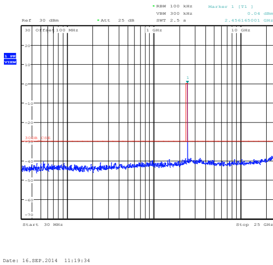
Figure 8.3-20: Conducted spurious emissions outside restricted bands for 802.11g, 54 Mbps, high channel
