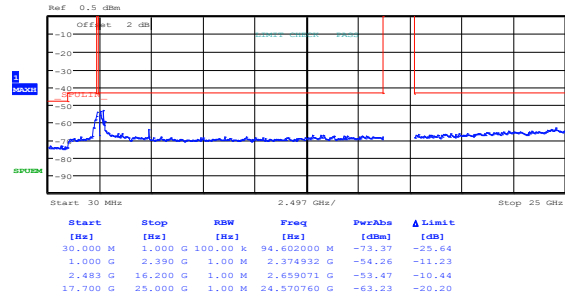
Figure 8.3-28: Conducted spurious emissions within restricted bands for 802.11g, 6 Mbps, mid channel
