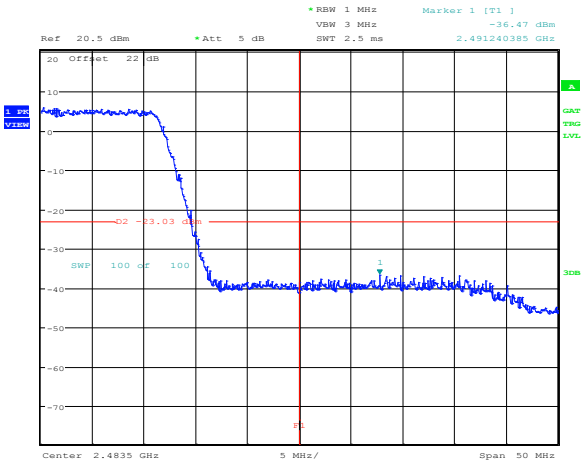
Figure 8.3-81: Band edge emission within restricted bands at 2.4835 GHz for 802.11n HT20, MCS 0, peak
