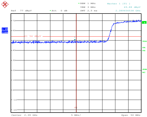
Figure 8.3-97: Cabinet radiation at the restricted band edge at 2.39 GHz for 802.11n HT20
