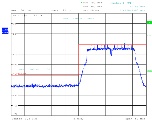
Figure 8.3-45: Band edge emission outside restricted bands at 2.4 GHz for 802.11b, 1 Mbps
