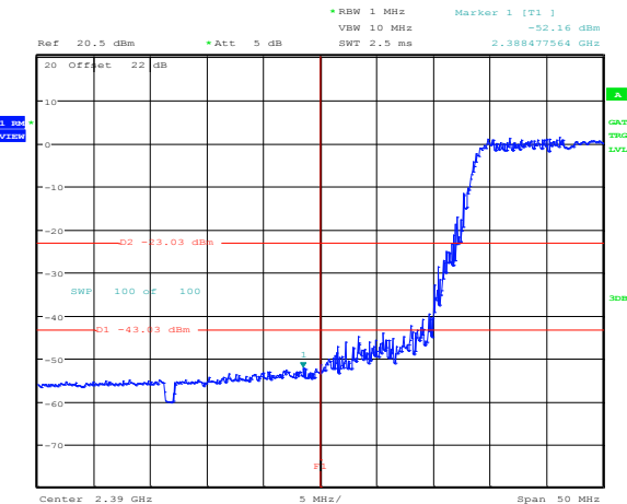
Figure 8.3-62: Band edge emission within restricted bands at 2.4 GHz for 802.11b, 1 Mbps, average
