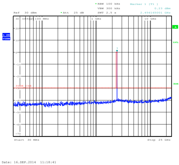
Figure 8.3-9: Conducted spurious emissions outside restricted bands for 802.11g, 6 Mbps, high channel
