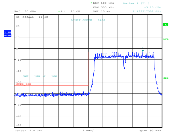
Figure 8.3-46: Band edge emission outside restricted bands at 2.4 GHz for 802.11g, 6 Mbps
