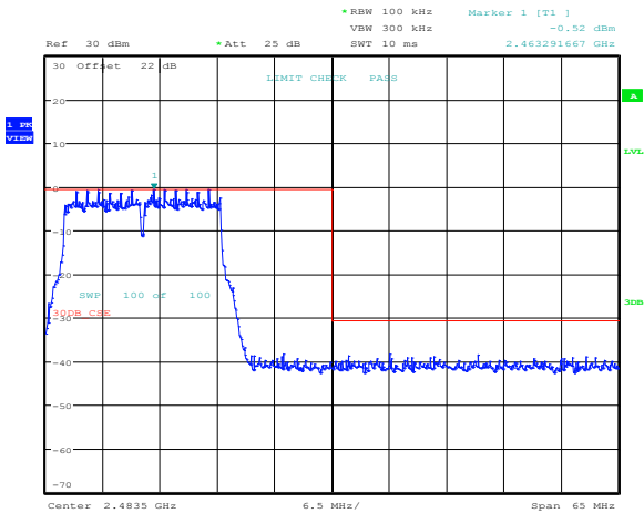
Figure 8.3-57: Band edge emission outside restricted bands at 2.4835 GHz for 802.11b, 11 Mbps
