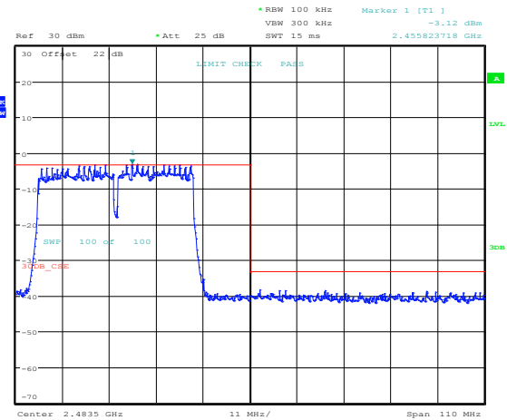
Figure 8.3-58: Band edge emission outside restricted bands at 2.4835 GHz for 802.11g, 54 Mbps
