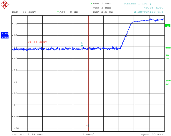
Figure 8.3-93: Cabinet radiation at the restricted band edge at 2.39 GHz for 802.11b
