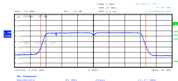
Figure 8.2-4: Output power on 802.11n HT40, sample plot
