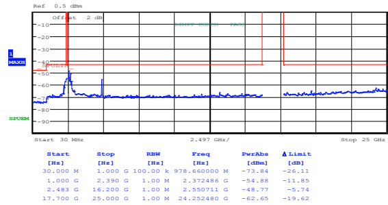
Figure 8.3-38: Conducted spurious emissions within restricted bands for 802.11b, 11 Mbps, mid channel
