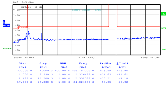
Figure 8.3-27: Conducted spurious emissions within restricted bands for 802.11b, 1 Mbps, mid channel
