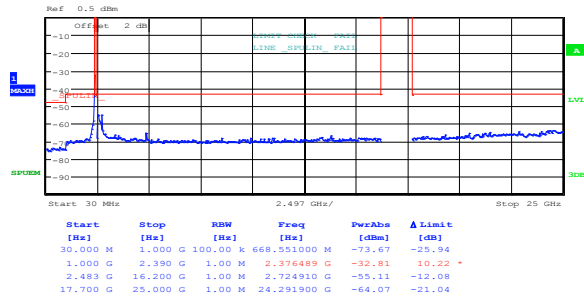
Figure 8.3-37: Conducted spurious emissions within restricted bands for 802.11n HT40, MCS 7, low channel
