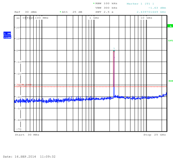
Figure 8.3-7: Conducted spurious emissions outside restricted bands for 802.11n HT20, MCS 0, mid channel
