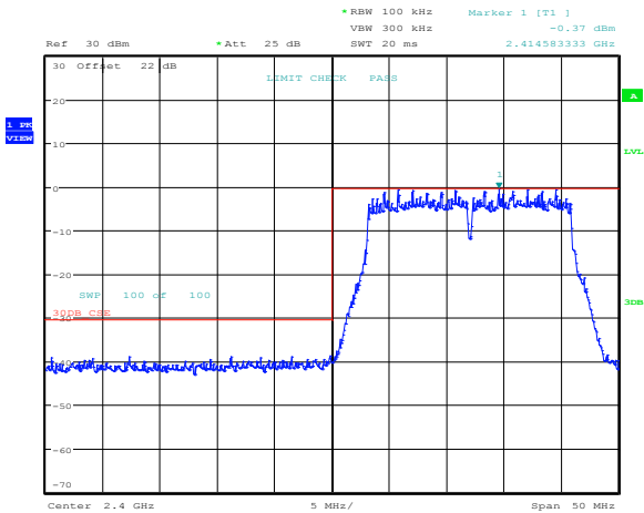
Figure 8.3-49: Band edge emission outside restricted bands at 2.4 GHz for 802.11b, 11 Mbps
