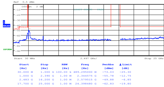
Figure 8.3-31: Conducted spurious emissions within restricted bands for 802.11g, 6 Mbps, high channel
