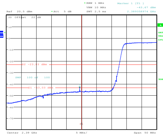
Figure 8.3-66: Band edge emission within restricted bands at 2.4 GHz for 802.11n HT20, MCS 0, average
