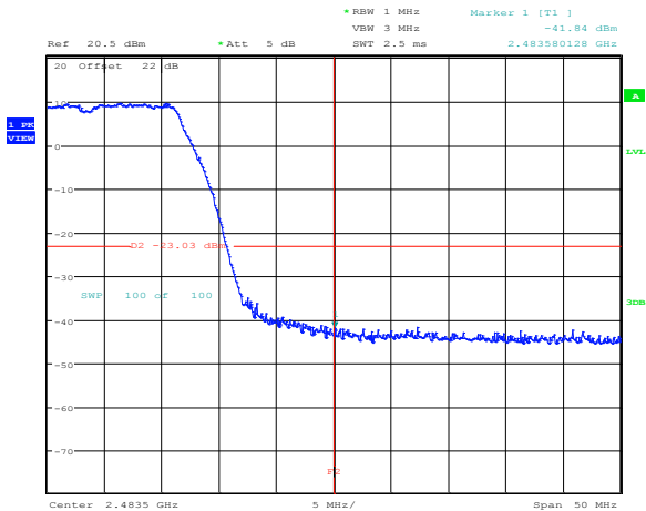
Figure 8.3-77: Band edge emission within restricted bands at 2.4835 GHz for 802.11b, 1 Mbps, peak
