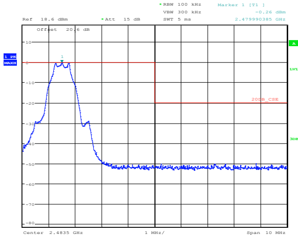
Figure 8.3-3: Conducted spurious emissions outside restricted bands, high channel
