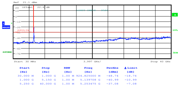
Figure 8.3-17: Spurious emissions outside restricted bands, 802.11ac VHT80, MCS 0
