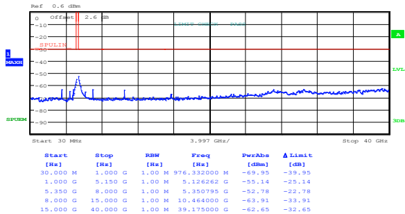
Figure 8.3-15: Spurious emissions outside restricted bands at high channel, 802.11ac VHT40, MCS 0
