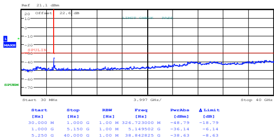
Figure 8.3-9: Spurious emissions outside restricted bands at low channel, 802.11n HT40, MCS 0
