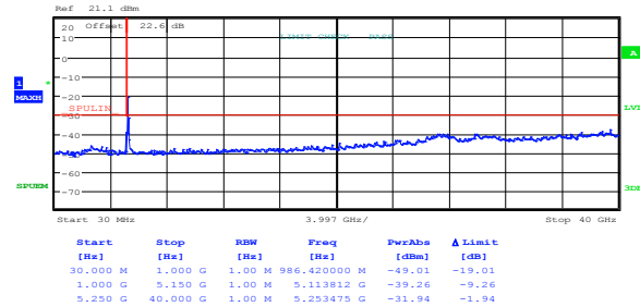
Figure 8.3-18: Spurious emissions outside restricted bands, 802.11ac VHT80, MCS 9
