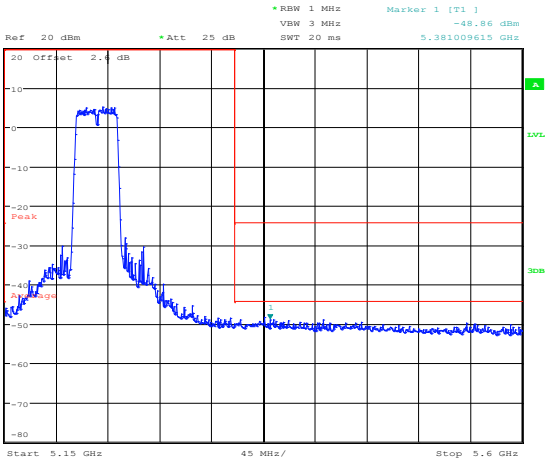
Figure 8.3-62: Upper band edge emission for 802.11n HT40 with MCS 7, peak
