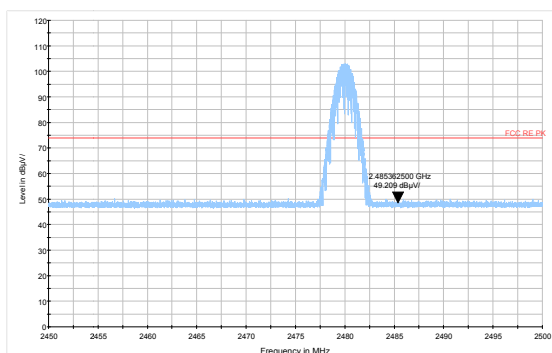
3DH5-Channel 78: Peak
