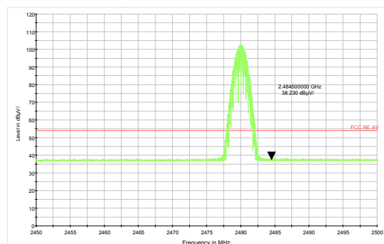
3DH5-Channel 78: Average
