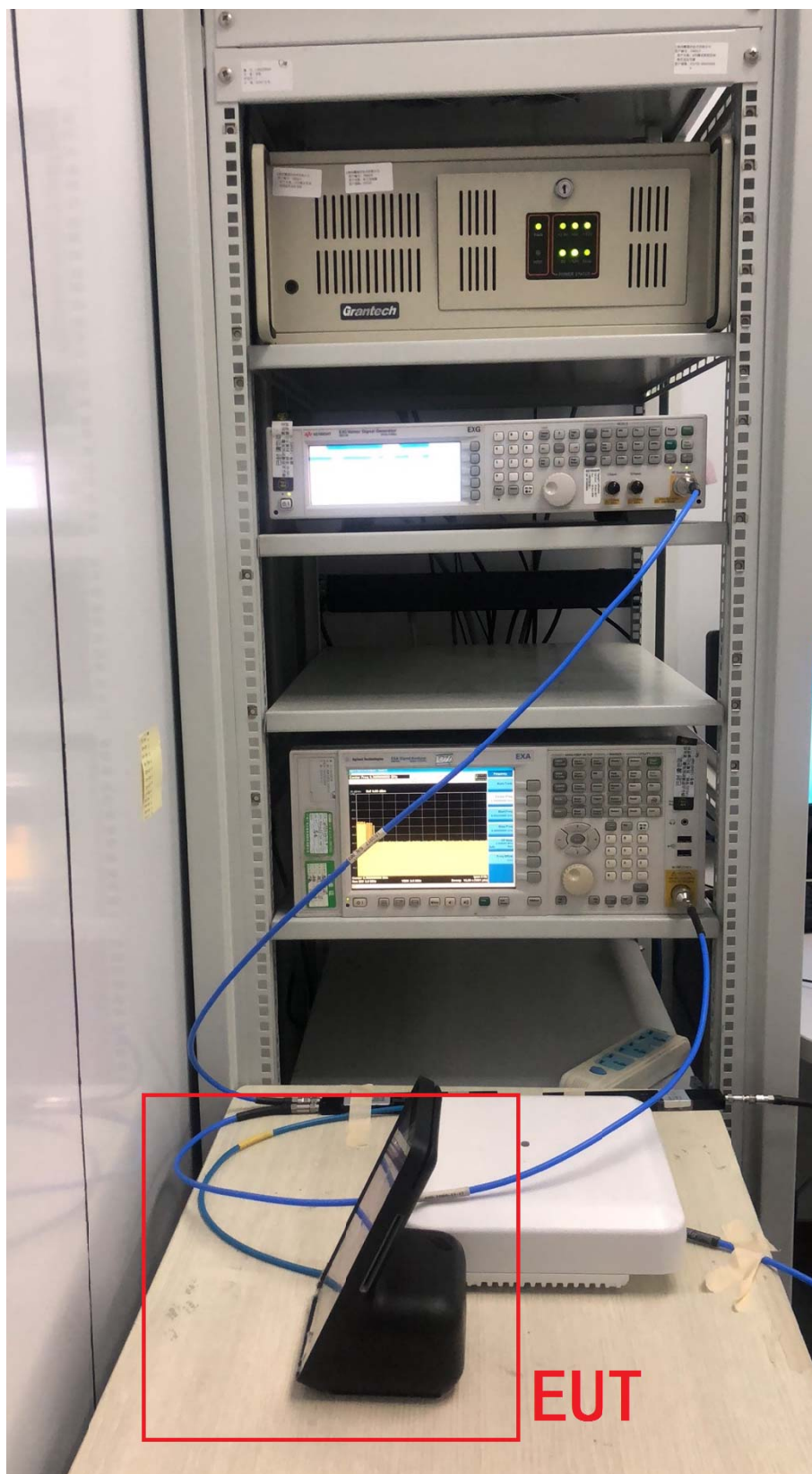
Picture 1 Test Setup
