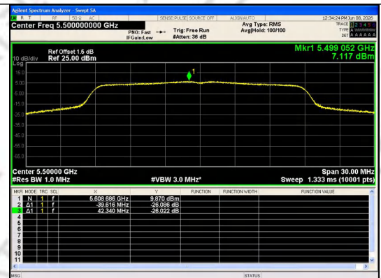
IEEE 802.11ac Channel 100 20MHz Antenna 1
