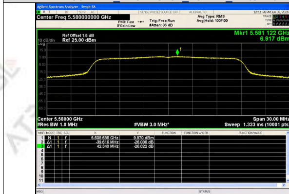
IEEE 802.11n Channel 116 20MHz Antenna 1
