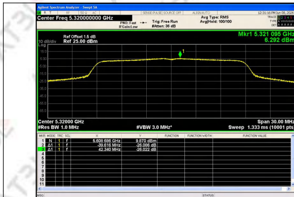
IEEE 802.11ac Channel 64 20MHz Antenna 1
