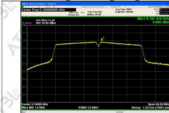
IEEE 802.11ac Channel 38 40MHz Antenna 1
