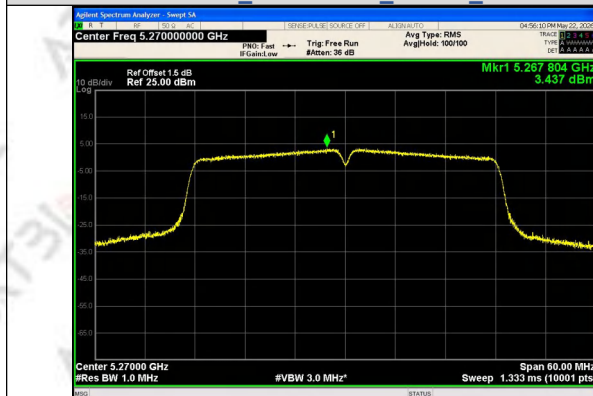
IEEE 802.11ac Channel 54 40MHz Antenna 1
