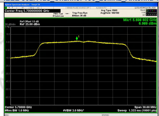
IEEE 802.11ac Channel 140 20MHz Antenna 1
