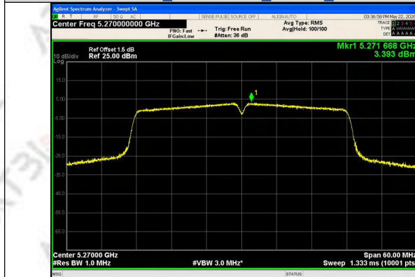
IEEE 802.11n Channel 54 40MHz Antenna 1
