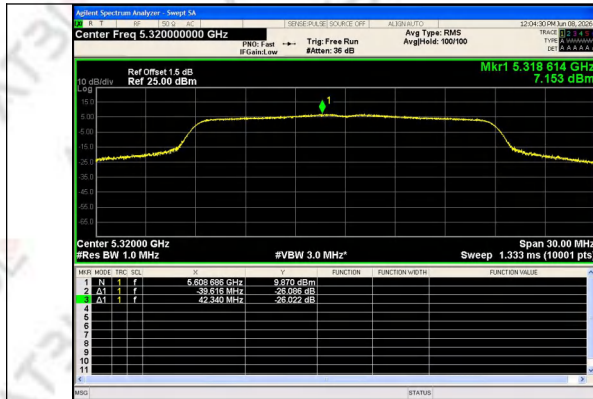
IEEE 802.11n Channel 64 20MHz Antenna 1
