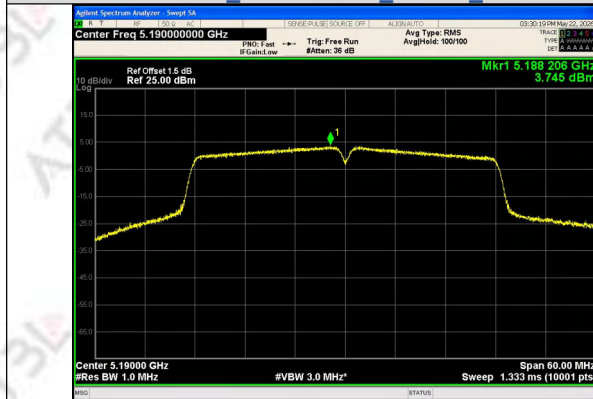
IEEE 802.11n Channel 38 40MHz Antenna 1
