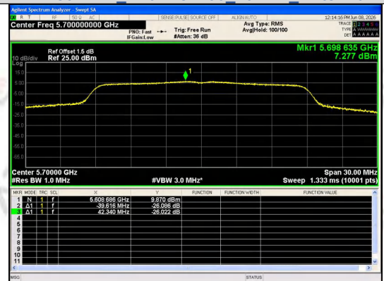
IEEE 802.11n Channel 140 20MHz Antenna 1
