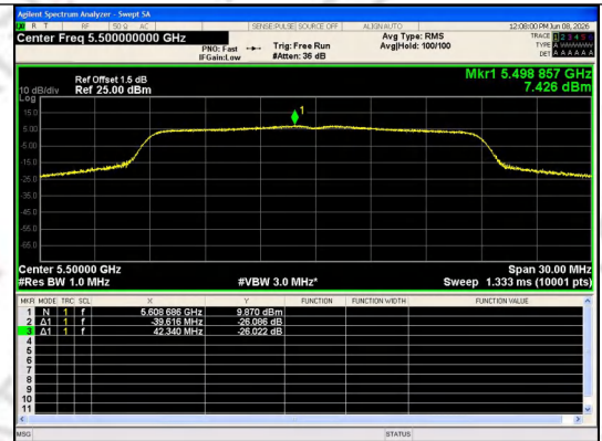
IEEE 802.11n Channel 100 20MHz Antenna 1
