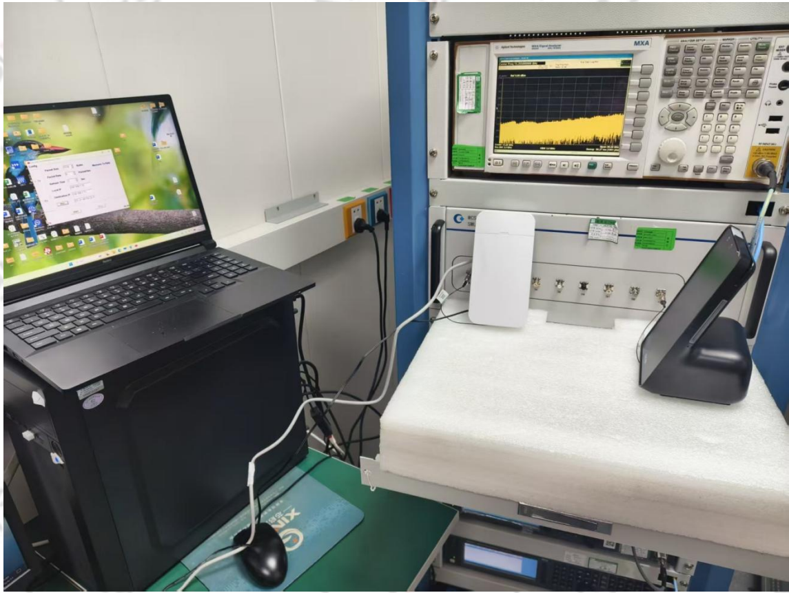
AC Power-Line Conducted Emission
