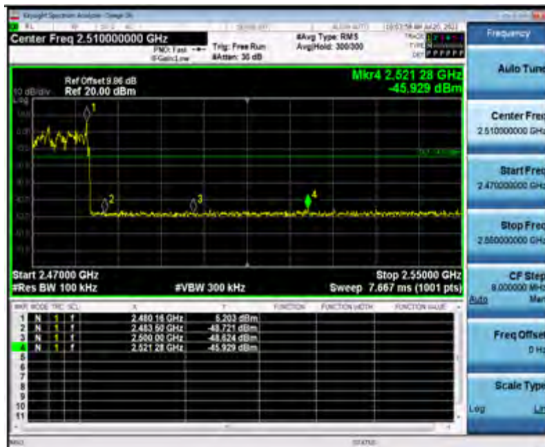
3DH5_High_2480
