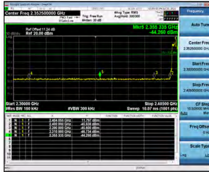
2DH5_Low_2402
