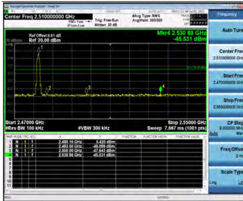
3DH5_High_2480
