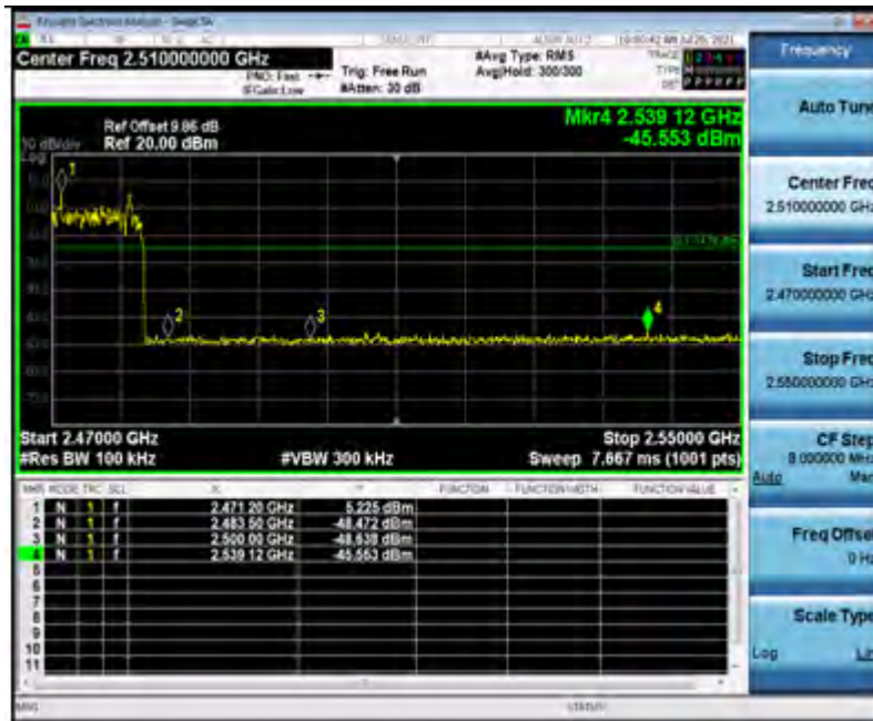
2DH5_High_2480
