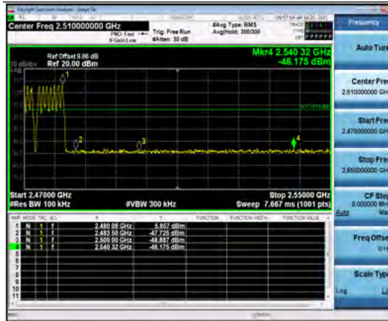
DH5_High_2480
