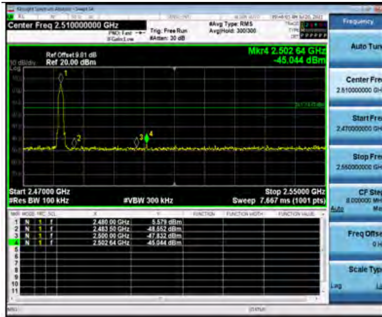
2DH5_High_2480
