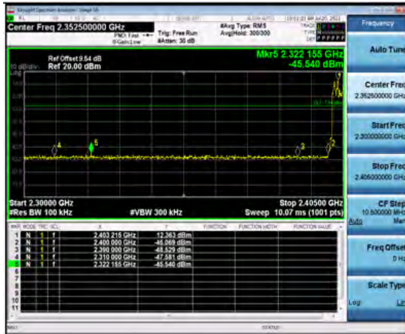
3DH5_Low_2402
