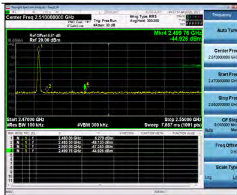
DH5_High_2480
