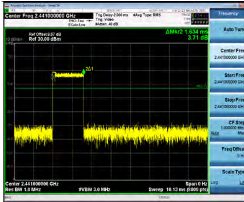
3DH3_Hop
