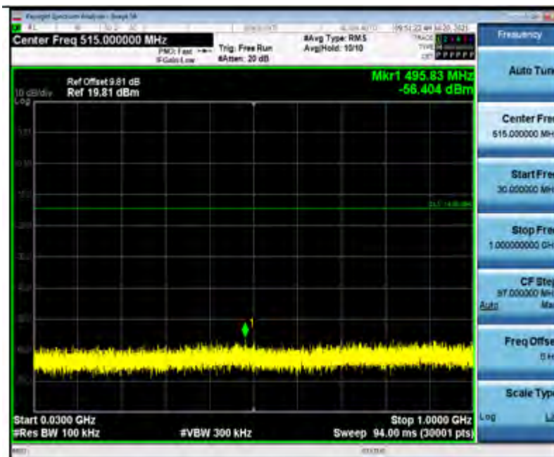
3DH5_2480_30~1000
