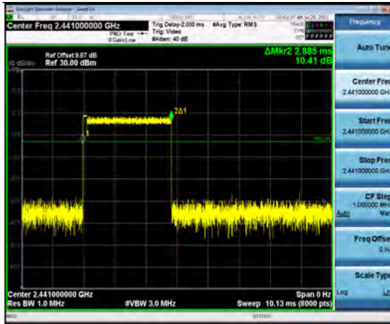
3DH5_Hop
