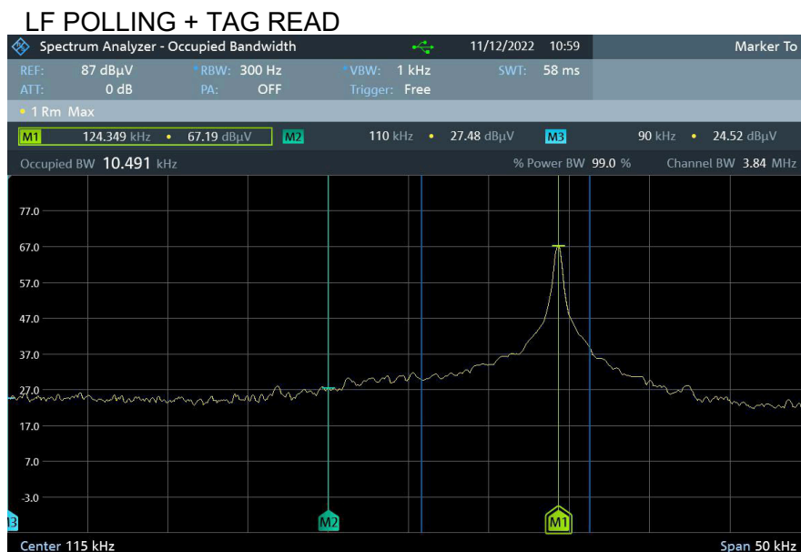
Figure 8: Example Intentional Emission Bandwidth.
